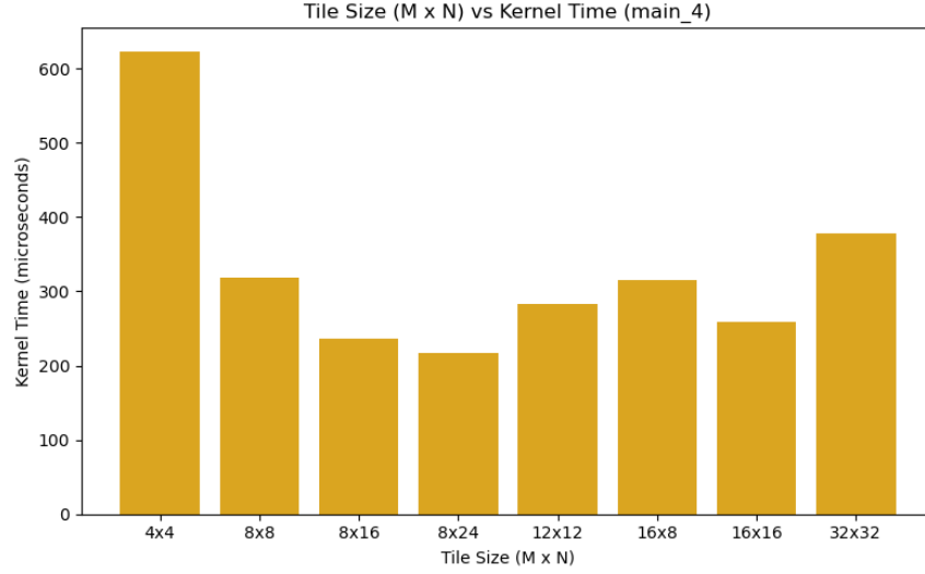
Figure 5: Performance for different tile sizes in tiled matrix transpose.
