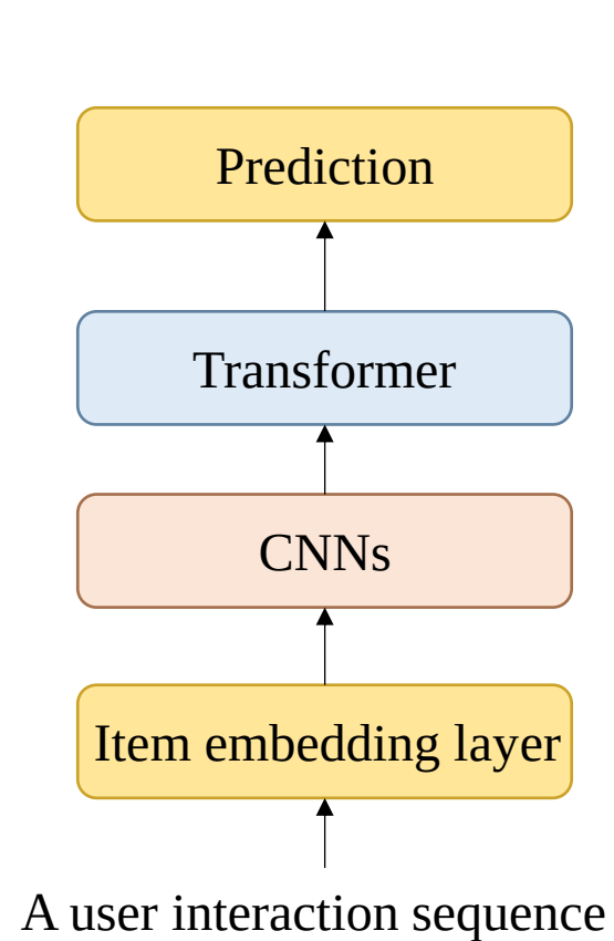
(b) CNNs and Transformer in cascade
