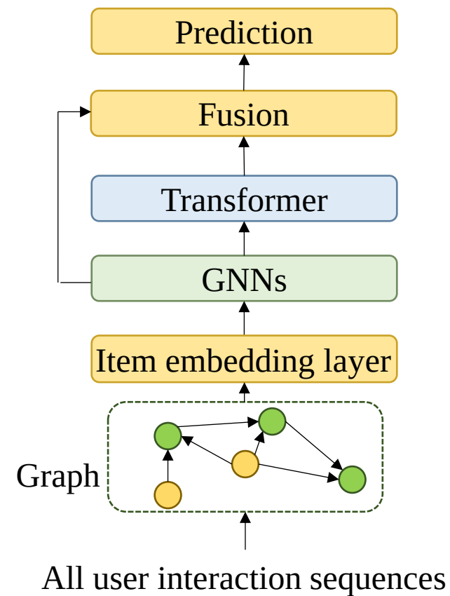
(c) GNNs and Transformer in cascade
