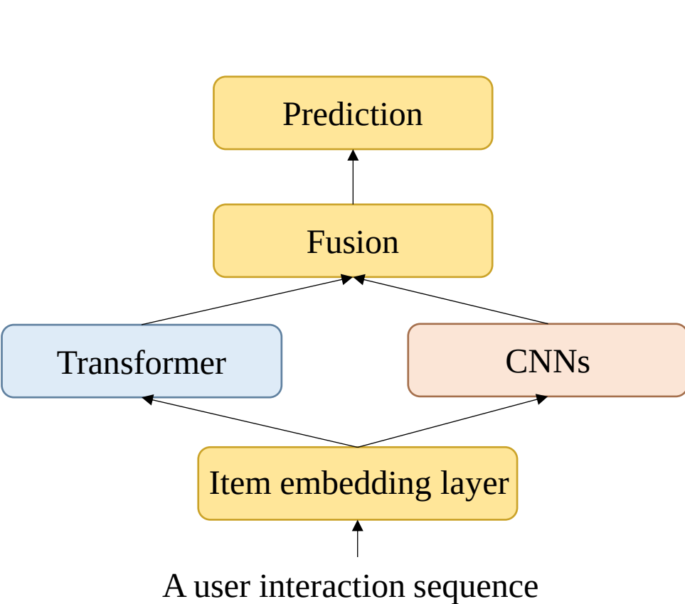
(a) CNNs and Transformer in parallel
