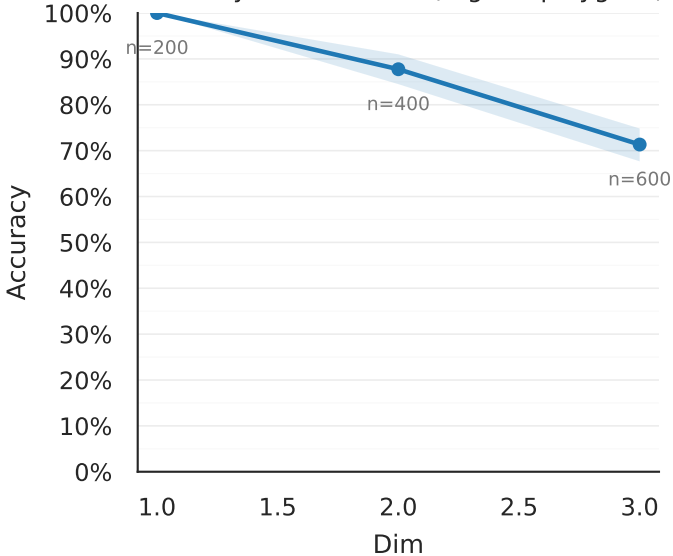
Accuracy vs dimension (regular polygons)
