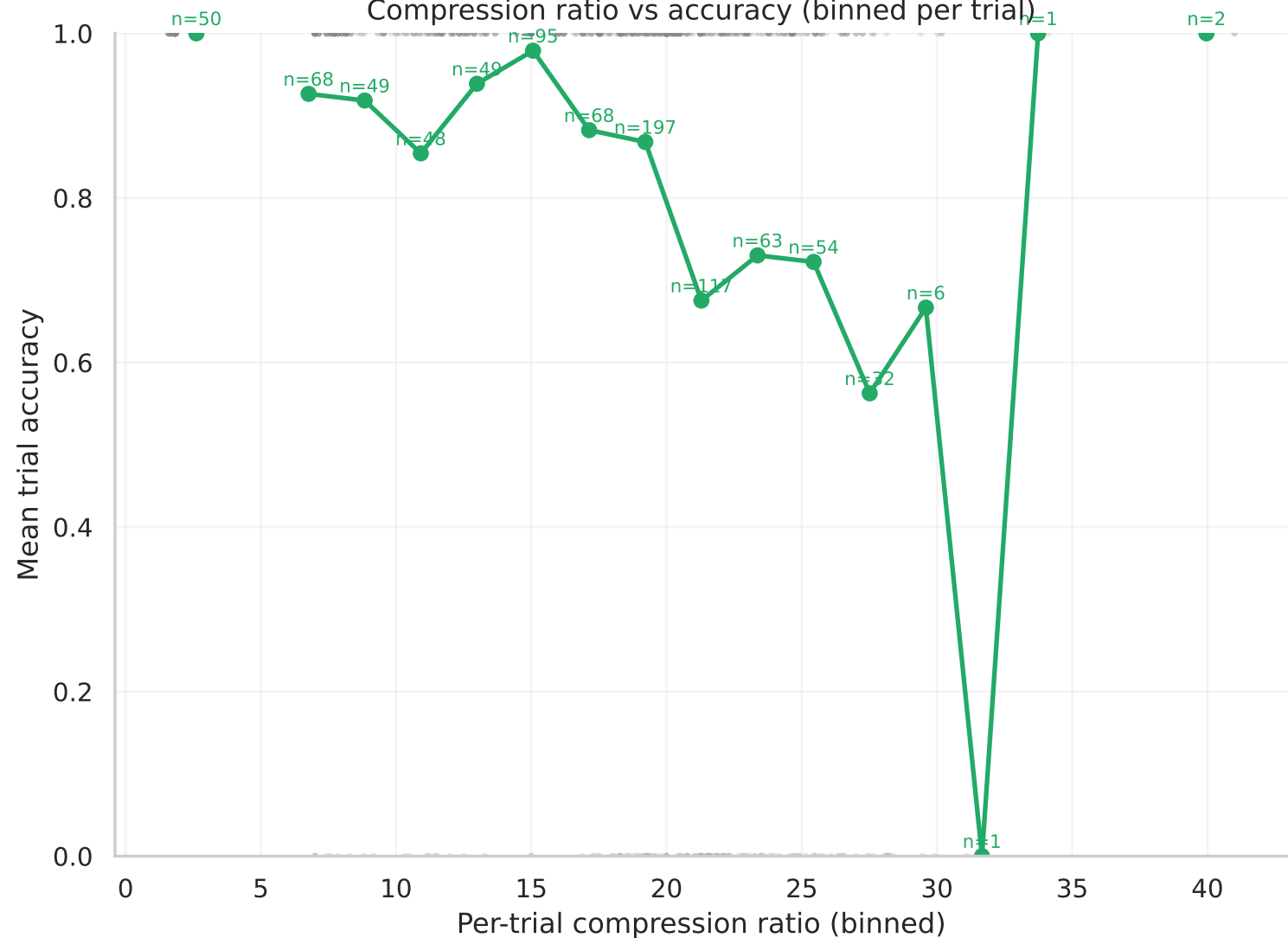
Compression ratio vs accuracy (binned per trial)
