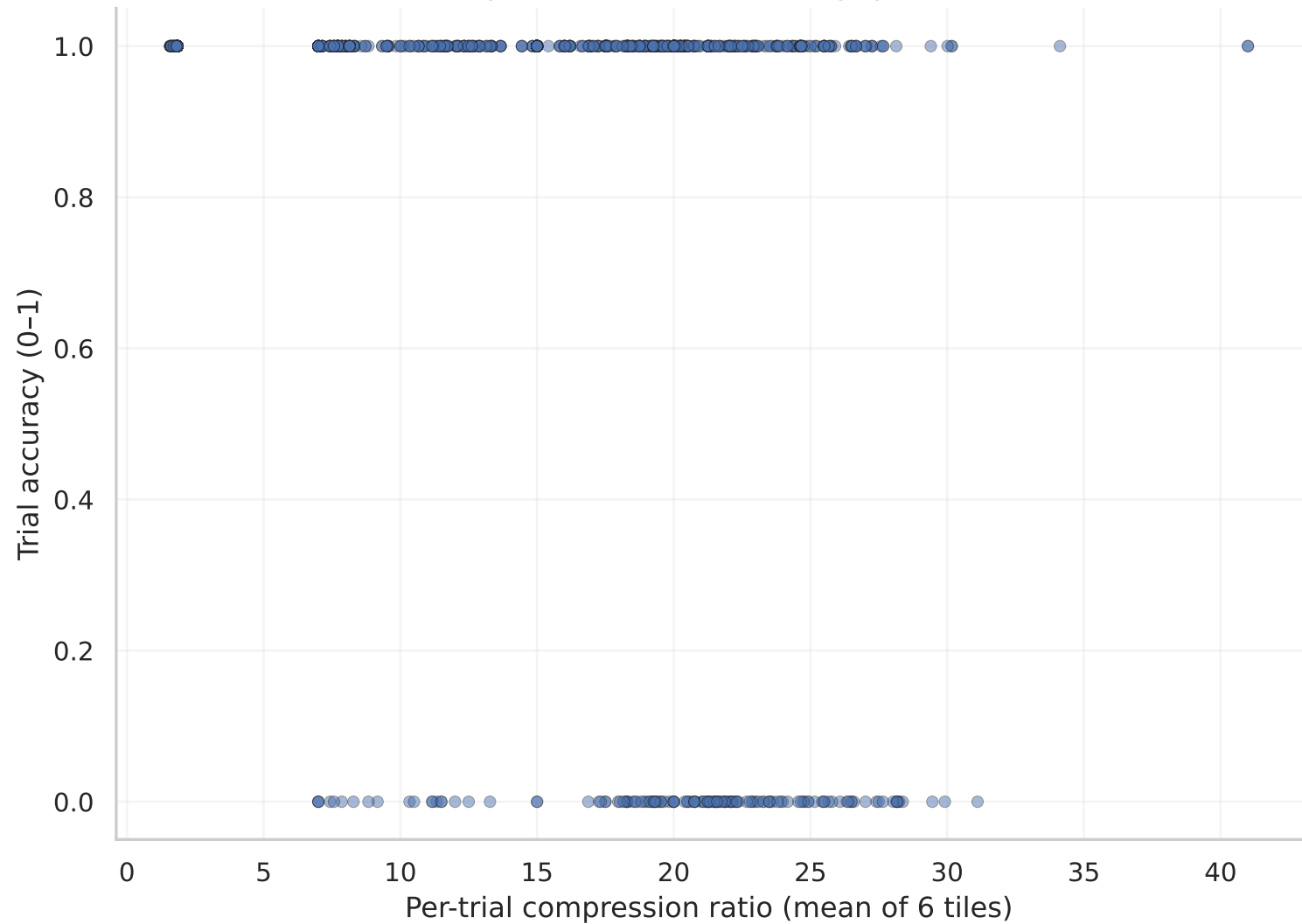
Compression ratio vs accuracy (per trial)
