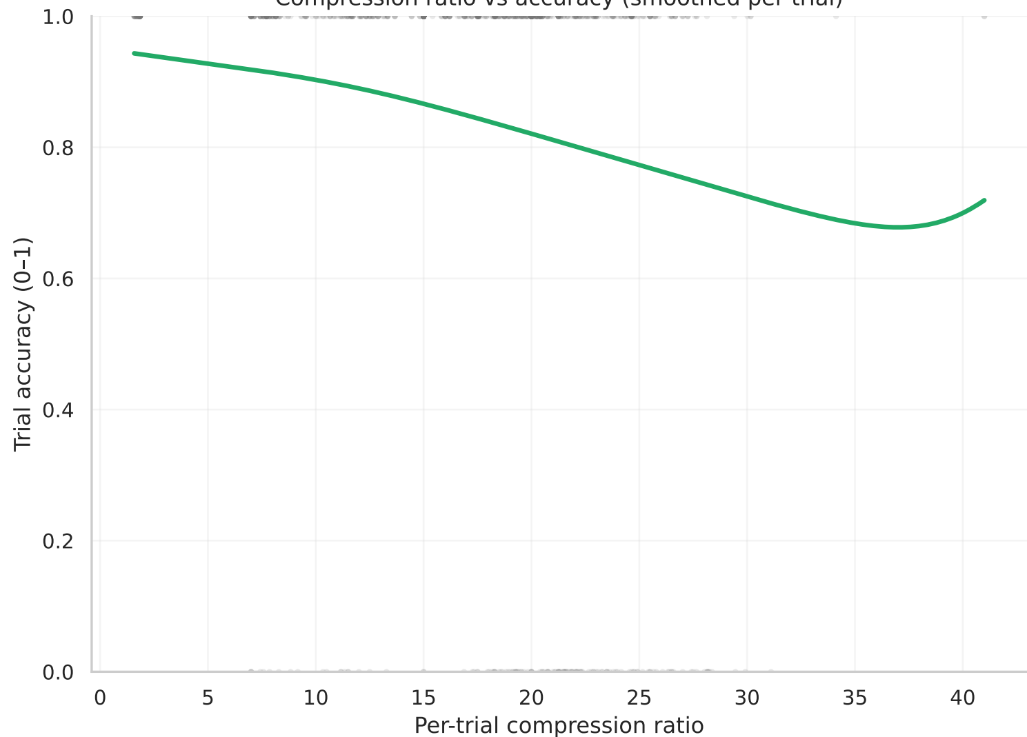
Compression ratio vs accuracy (smoothed per trial)
