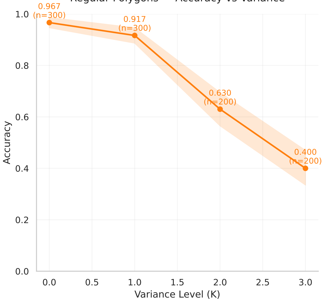
Regular Polygons — Accuracy vs Variance
