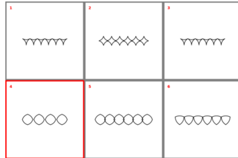
dim 3 | var 2 | polygons
