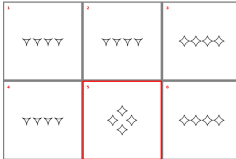
dim 2 | var 1 | polygons
