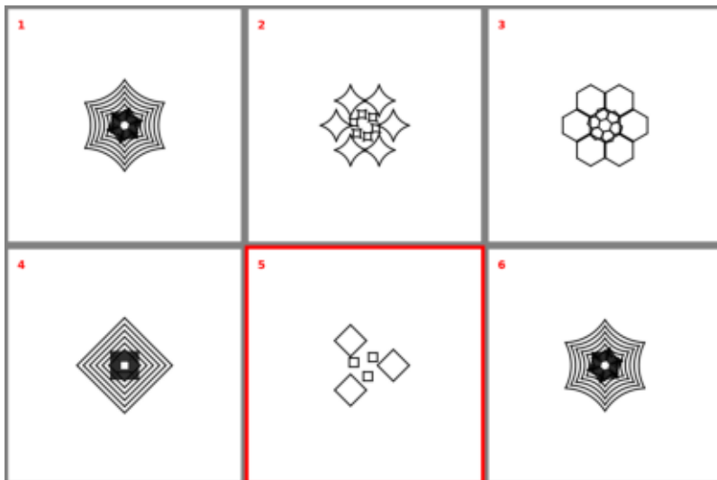
var 3 | dim 3 | polygons
