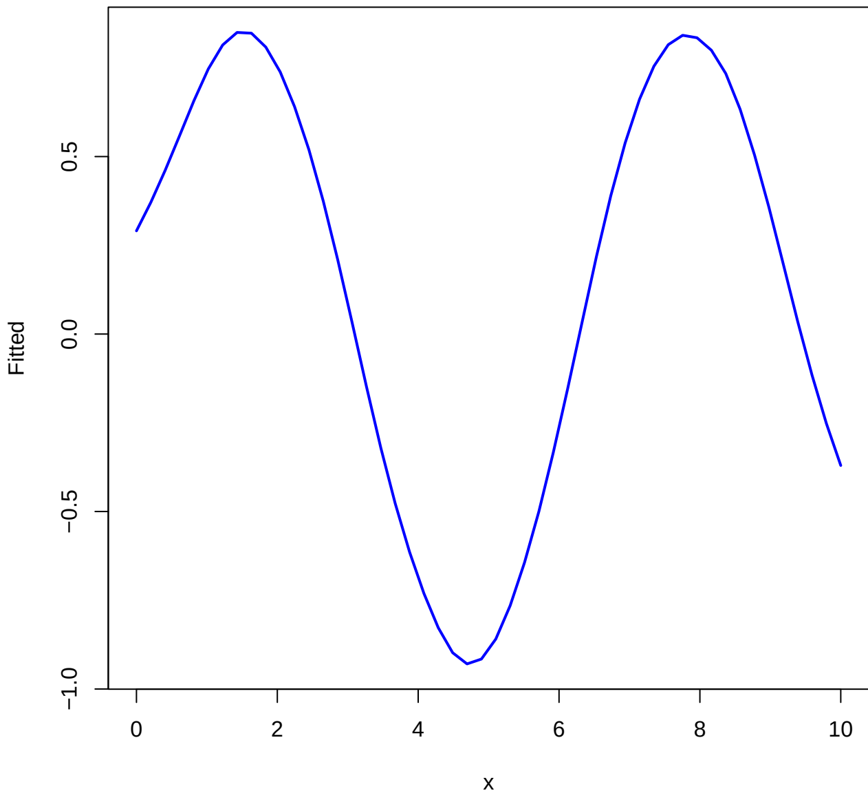
LOWESS Fit
