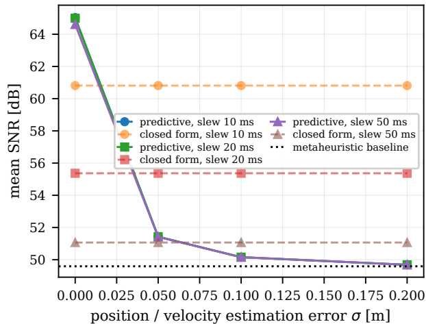
Sensitivity to tracking accuracy
