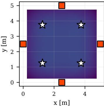
Conventional (no IRS) 43.7 – 51.0 dB
