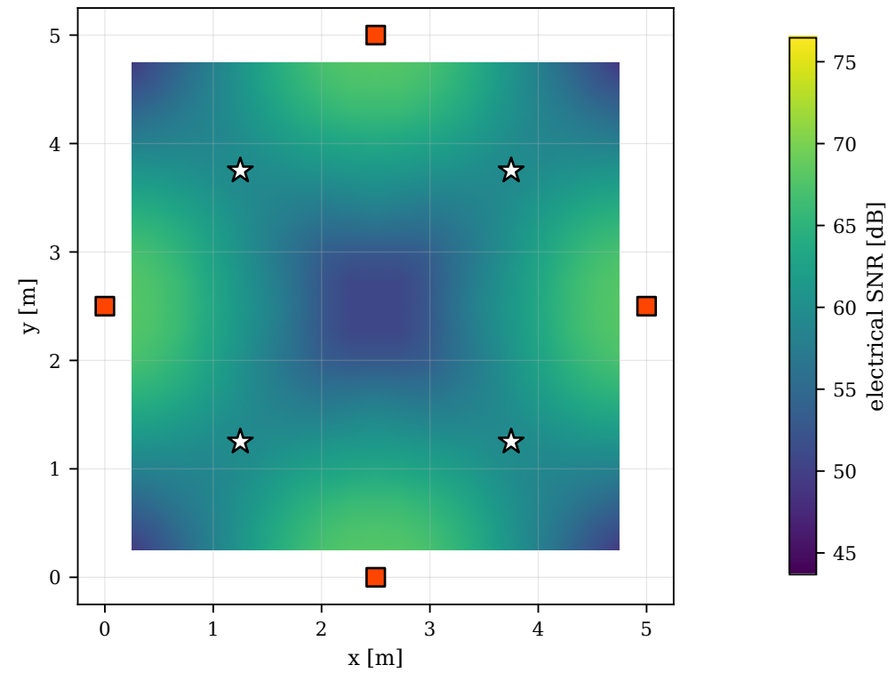
IRS, specular reflection 49.4 – 67.8 dB
