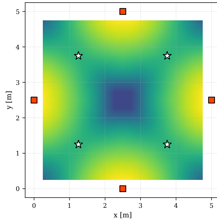
IRS, base-paper cosine model 50.7 – 76.5 dB
