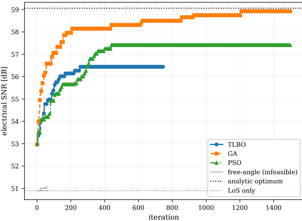
Convergence per iteration
