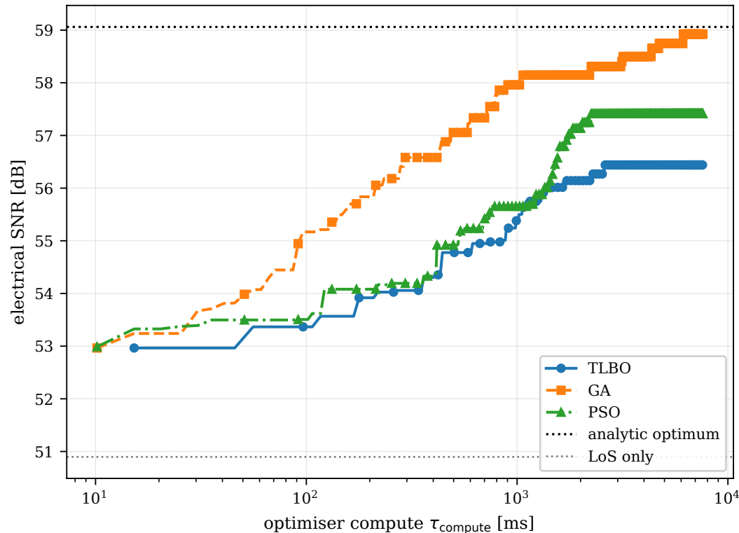
Convergence per unit compute
