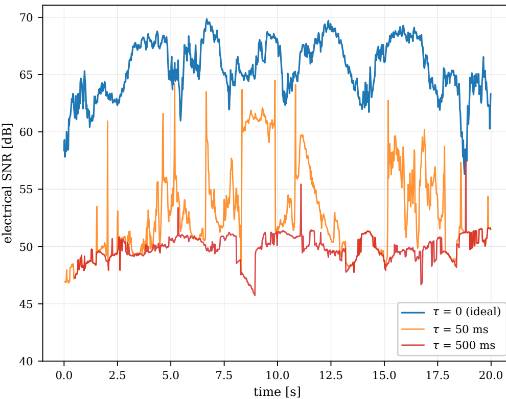
Specular, walking 1.0 m/s, one trace
