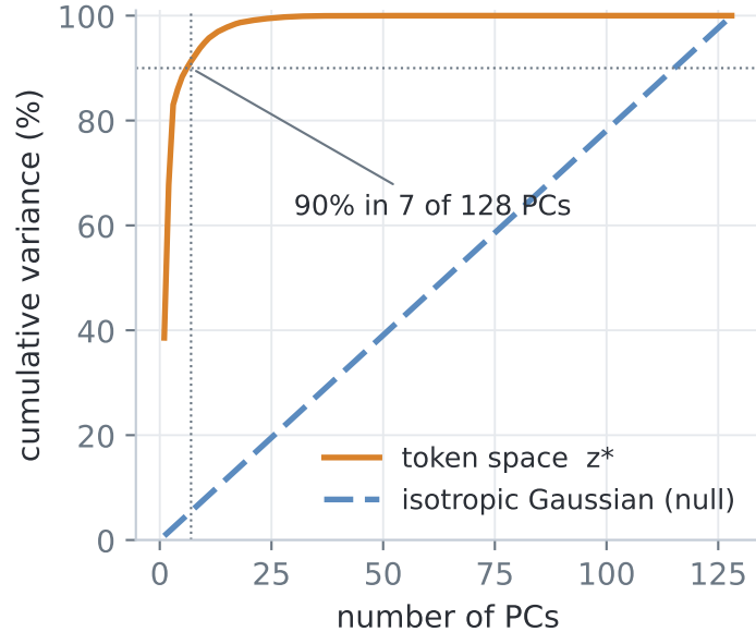
B Variance concentration
