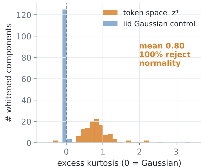
C Non-Gaussian tails
