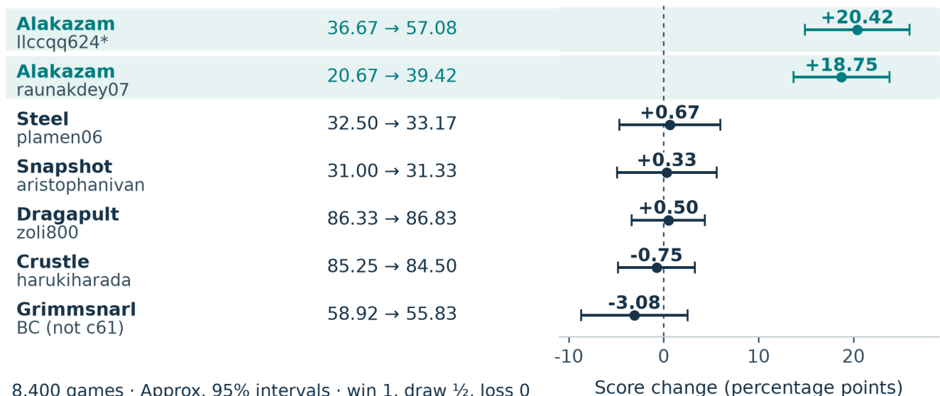
Figure 2. A later panel of seven implementations, 600 games per arm per opponent, balanced by seat. Intervals condition on these implementations and independent games.
