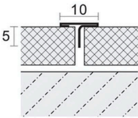
DM-STP145-10W
