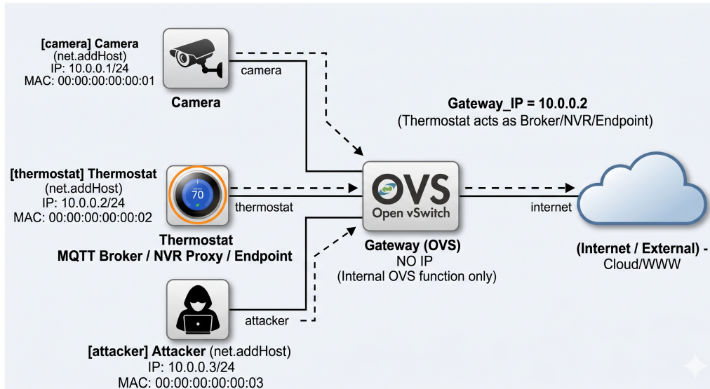
Figure 7: Home IoT Network Design
