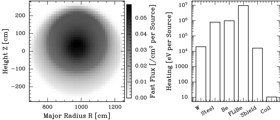
Figure 9: Volumetric flux tally on the conformal blanket (device 59509, scattering on, native StellaratorSource ). Left: poloidal fast-flux ( E > 0.1 MeV) distribution ( \phi -averaged), concentrated in the plasma-facing region and attenuating outward through the blanket. Right: heating deposited per blanket layer (per source neutron), dominated by the FLiBe breeder.
