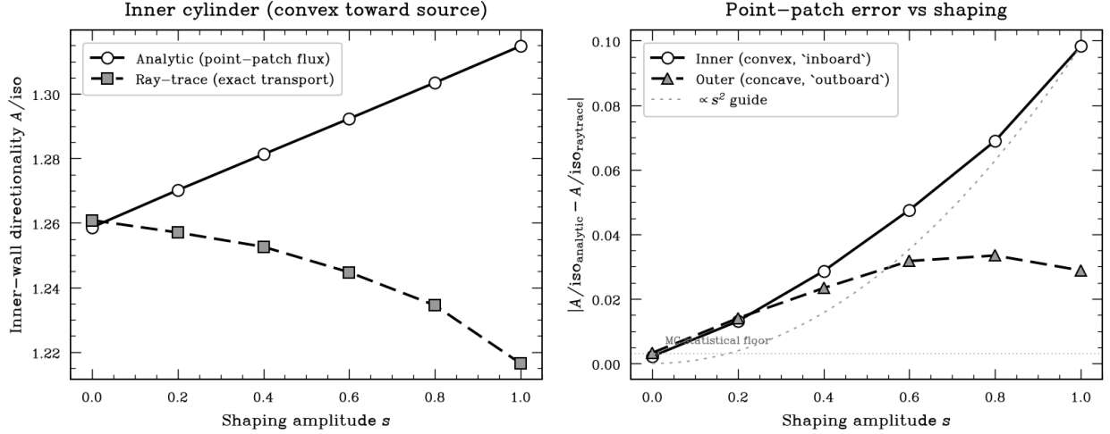
Figure 3: Single-filament demonstration that the inboard residual is the analytic point-patch limit. Left: inner-wall directionality A/\text{iso} from the analytic point-patch flux integral and from exact ray-tracing of the same births, versus the shaping amplitude s ; coincident for an axisymmetric source ( s = 0 ) and diverging as s grows. Right: the analytic \leftrightarrow ray-trace discrepancy versus s for the convex inner (inboard) and concave outer (outboard) cylinders, with an s^2 guide.
