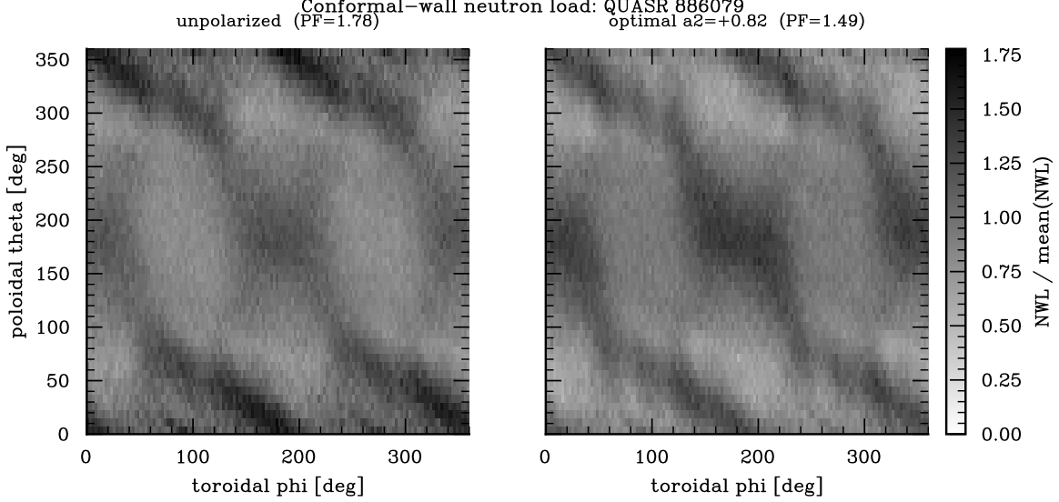
Figure 7: Neutron wall load \text{NWL}/\overline{\text{NWL}} on the DAGMC conformal first wall of QUASR device 886079 (real free-streaming StellaratorSource transport): unpolarized (left) versus peaking-optimal polarization a_2 = +0.82 (right). The peaking factor falls only from 1.78 to 1.49: the near-field hot spot is not steerable, though the broad load is visibly redistributed.
