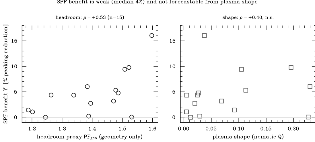
Figure 8: The polarization steering benefit is weak and not forecastable from plasma shape ( n = 15 conformal-wall devices). Left: the benefit correlates only weakly with a transport-free isotropic peaking (headroom) proxy ( \rho = +0.53 , borderline at n = 15 ). Right: it does not correlate with a pure-plasma shape metric ( \rho = +0.40 , not significant). The steering benefit must be evaluated per device by transport.
