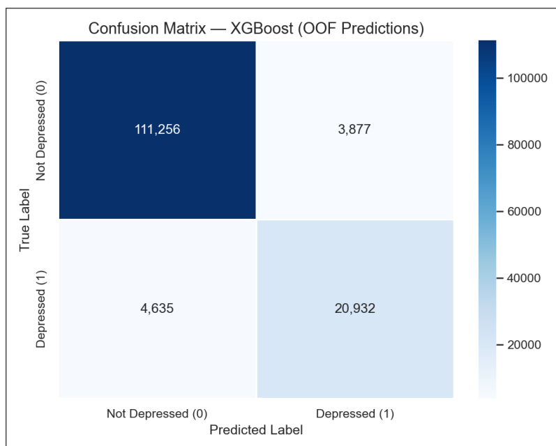
Hình 16: Confusion Matrix — XGBoost (OOF Predictions)
