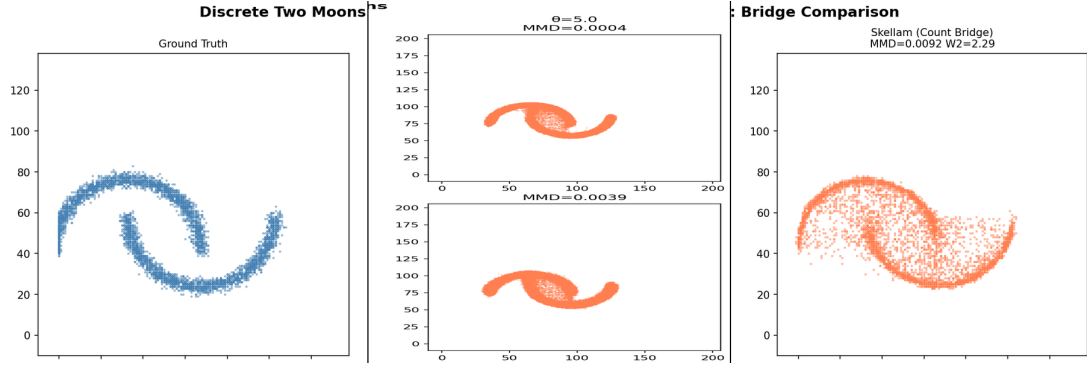
Figure 1: Visual Apples-to-Apples Evaluation. Left: Target Topology — Center: Generative Moran ( N = 200, \theta = 5.0 ) — Right: Baseline Count Bridge. Notice the absolute structural tightness achieved naturally globally minimizing continuous margins.
