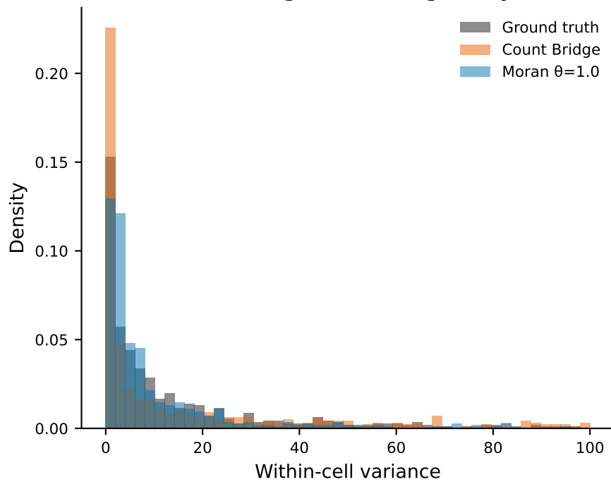
(B) Biological Heterogeneity
