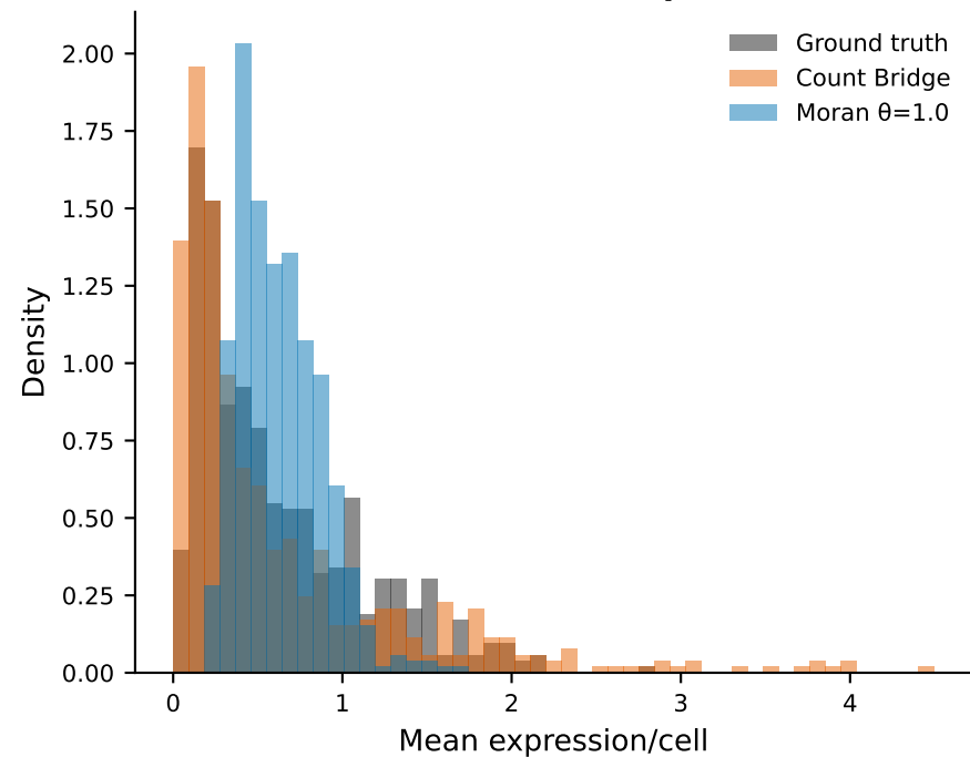
(A) Per-Cell Mean Expression
