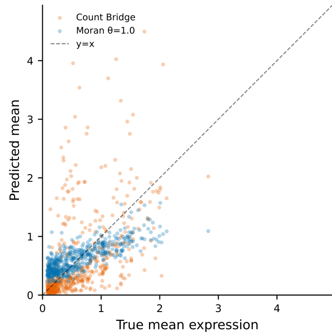
(C) Predicted vs True
