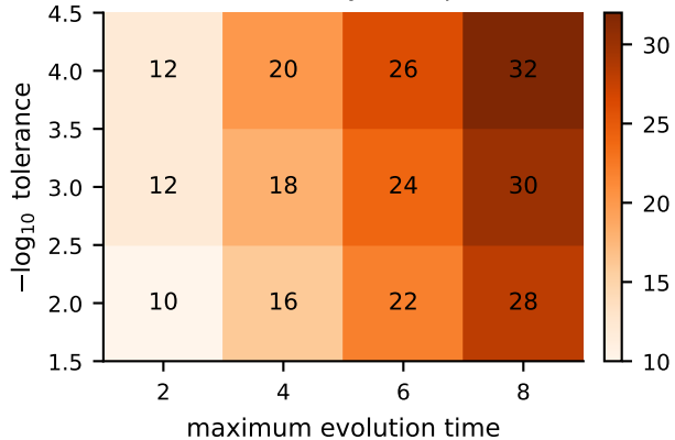
selected Krylov depth
