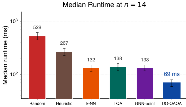
FIG. 3. Median wall-clock runtime at n=14 on a logarithmic scale.
