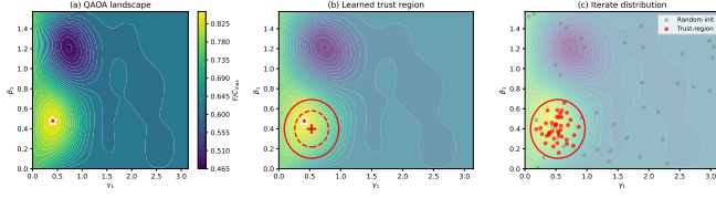
FIG. 1. Trust-region mechanism on an n=8 Erdős-Rényi instance at p=2 (layer-1 slice). (a) Landscape of the QAOA objective, with the optimum marked by a star. (b) Learned Mahalanobis trust regions at 95% (solid) and 68% (dashed), concentrated around the high-quality basin. (c) Random initializations (gray) versus trust-region samples (red), showing that the learned ellipsoid concentrates evaluations near the optimum.
