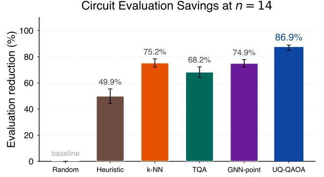
FIG. 6. Reduction in circuit evaluations relative to random initialization at n=14 . The random-initialization baseline is normalized to 0%, so each bar reports the fraction of hardware queries avoided by replacing uninformed initialization with a learned initialization strategy.
