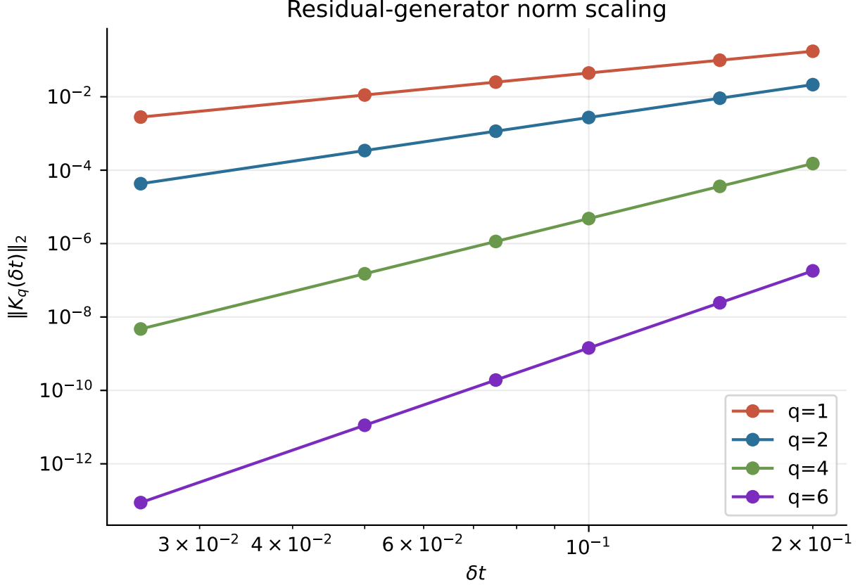
FIG. 8. Residual-generator norm versus step size for n = 4 and q = 1, 2, 4, 6 . The norm decreases rapidly with order, consistent with product-formula order conditions and Theorem 3.
