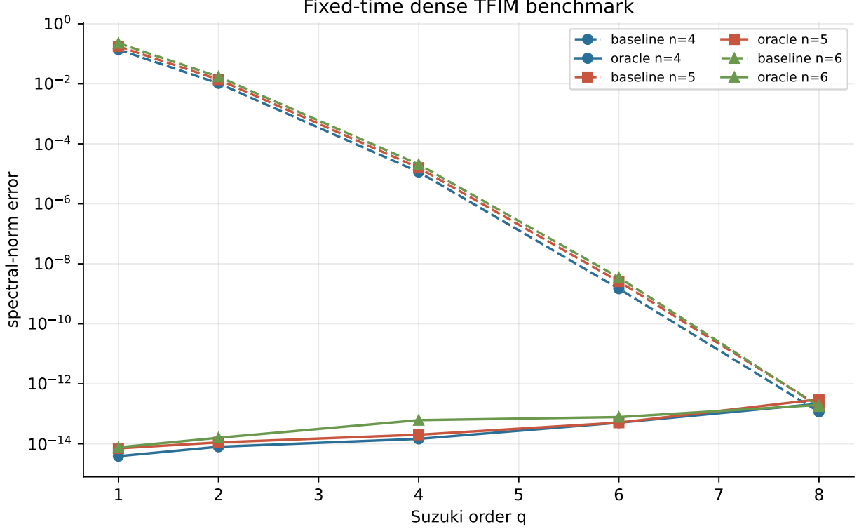
FIG. 3. Fixed-time spectral-norm errors for n = 4, 5, 6 and q = 1, 2, 4, 6, 8 . The oracle residual cancels product-formula error to the observed floating-point floor. The highest-order baseline is itself near round-off at this step size.
