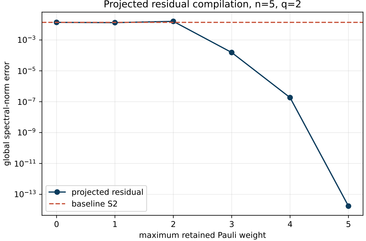
FIG. 4. Projected residual error versus maximum retained Pauli weight for n = 5 , q = 2 . The sharp improvement at w = 3 is predicted by the leading-support theorem for the Strang residual.
