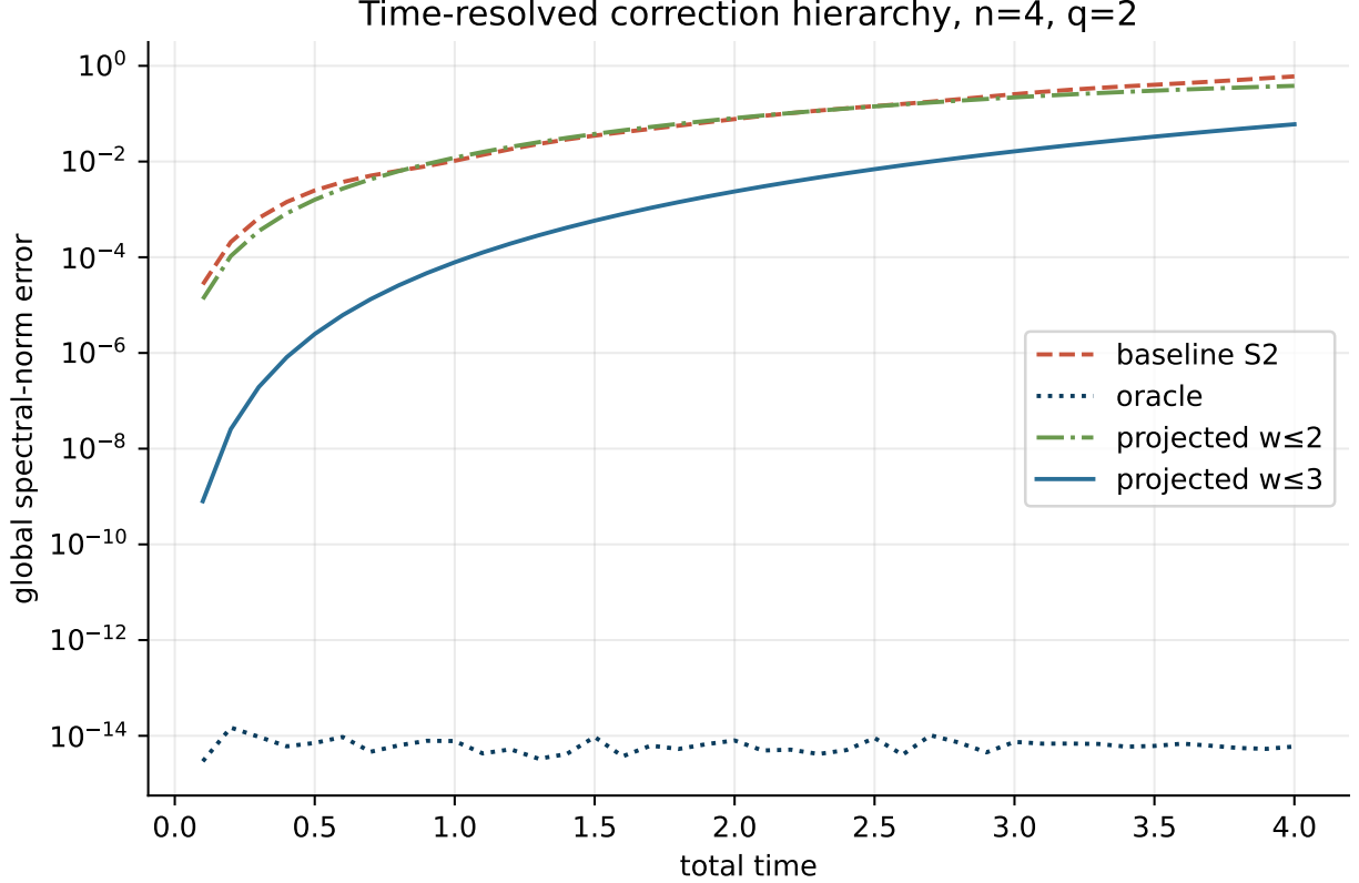
FIG. 5. Time-resolved correction hierarchy for n = 4 , q = 2 , J = h = 1 , and r = 10 . The w \leq 3 projected residual uniformly improves the baseline in this sweep; w \leq 2 is less reliable.
