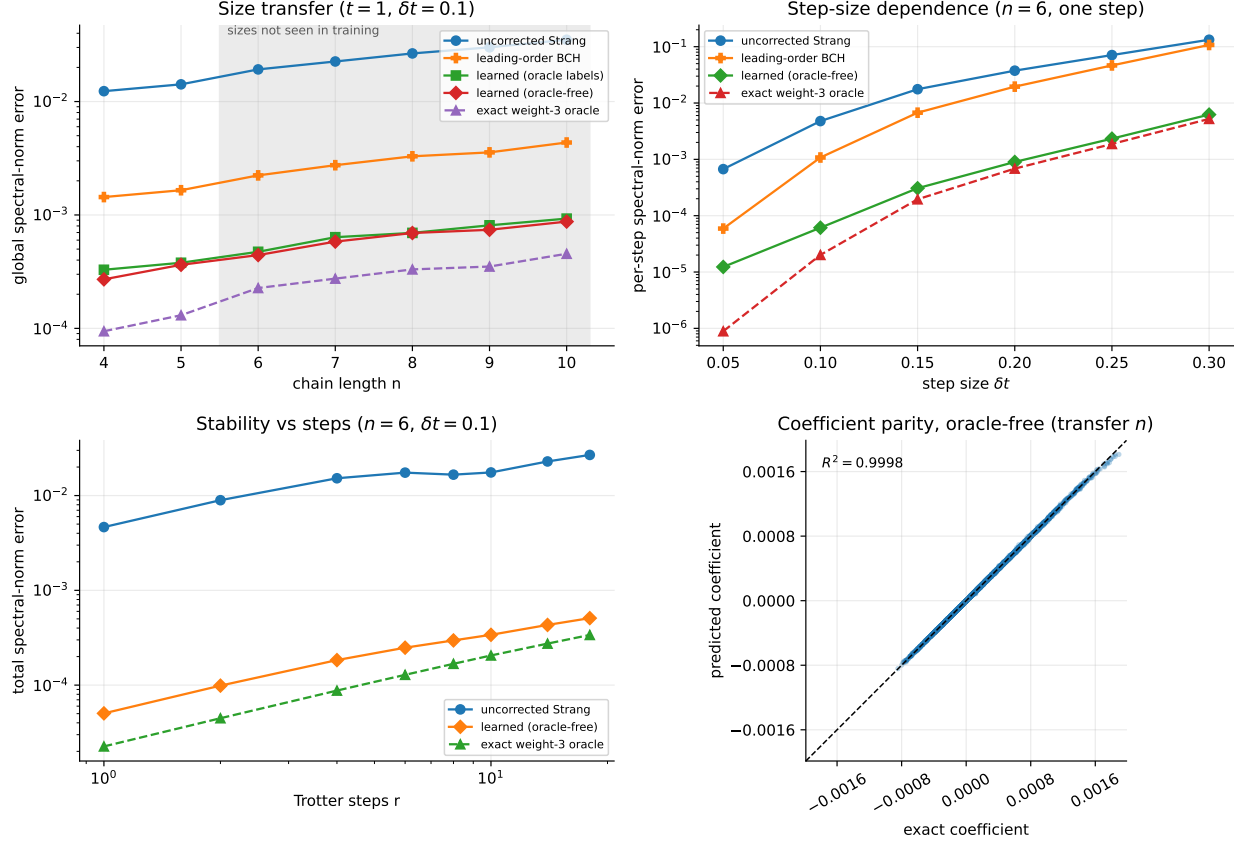
FIG. 9. Learned residual generators on the disordered TFIM. Top left: global spectral-norm error at t = 1 , \delta t = 0.1 versus chain length for the uncorrected Strang step, leading-order BCH, the learned correction trained on oracle labels and on oracle-free patch labels (overlapping), and the exact weight- \leq 3 oracle; the shaded region marks lengths absent from training ( n > 5 ), extending to n = 10 . Top right: per-step error versus step size \delta t at n = 6 ; leading-order BCH approaches the uncorrected step as \delta t grows, while the learned correction tracks the oracle. Bottom left: total error versus number of Trotter steps r ( n = 6 , \delta t = 0.1 ), growing linearly in r as Theorem 4 predicts. Bottom right: oracle-free predicted versus exact coefficients on held-out transfer sizes n = 6, \dots, 10 ( R^2 = 0.9998 ). One per-site network, trained only on n = 4, 5 , sees only local couplings at inference.
