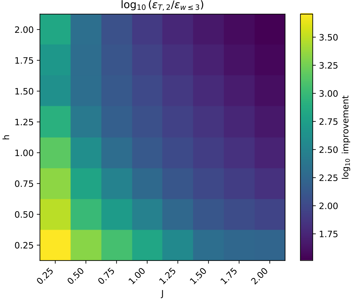
FIG. 6. Parameter-space improvement ratio for the w \leq 3 projected residual, plotted as \log_{10}(\epsilon_{T,2}/\epsilon_{w \leq 3}) . All 64 deterministic grid points improve over the baseline.
