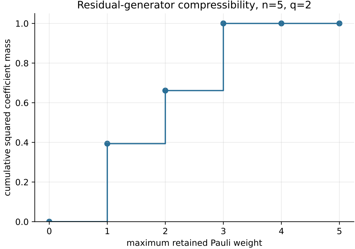
FIG. 7. Cumulative squared Pauli coefficient mass for the n = 5 , q = 2 residual generator. Weight three captures the dominant leading structure; higher weights capture subleading BCH terms.
