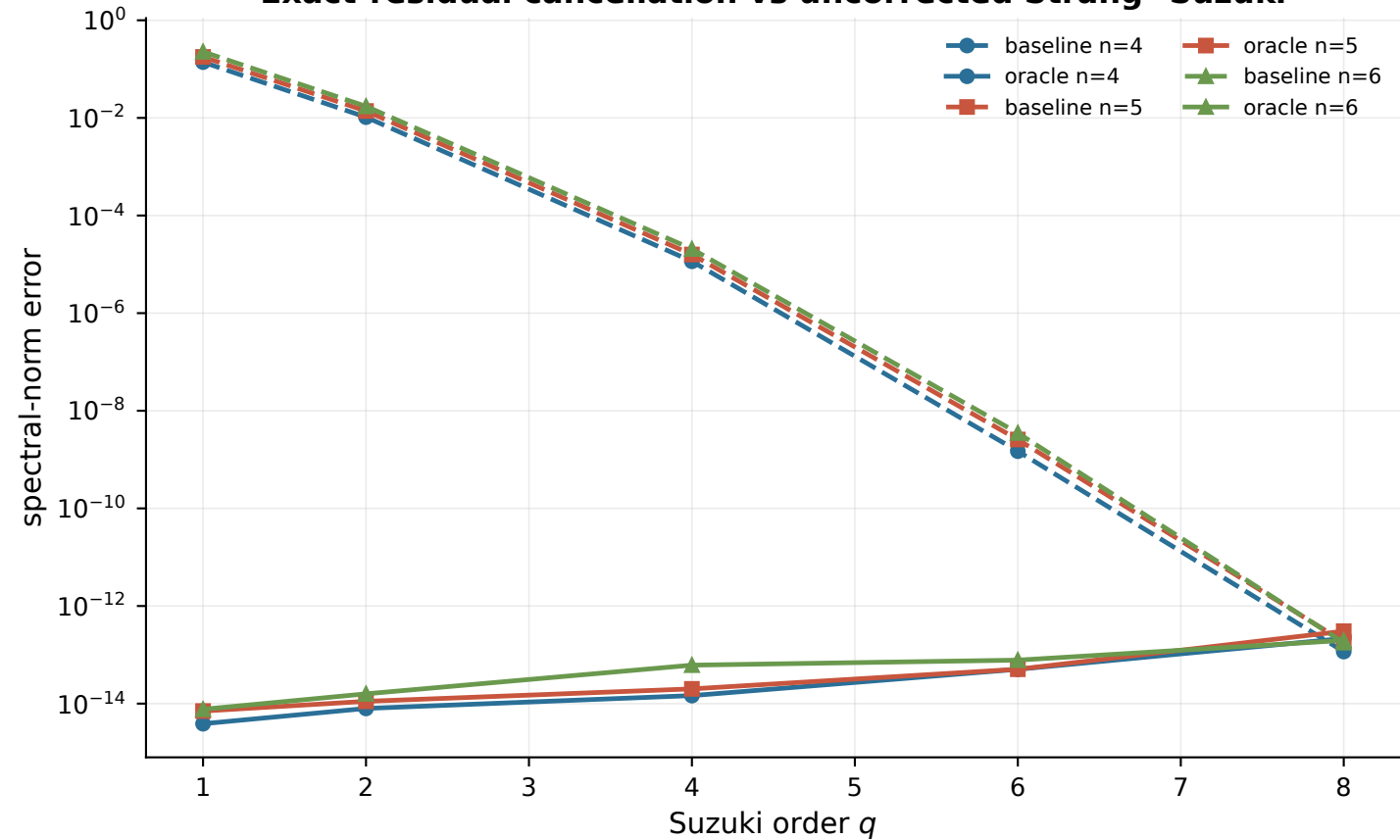
Exact-residual cancellation vs uncorrected Strang--Suzuki
