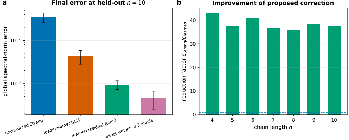
Figure 3. Proposed learned correction versus all baselines. a , Final global spectral-norm error at the largest held-out transfer size ( n = 10 ) for the uncorrected Strang step, leading-order BCH, the learned residual (ours), and the exact weight- \leq 3 oracle; error bars show one standard deviation over disordered realizations. b , Error-reduction factor \epsilon_{\text{Strang}}/\epsilon_{\text{learned}} of the learned correction over the uncorrected Strang baseline across all chain lengths, including the held-out transfer sizes n \geq 6 .
