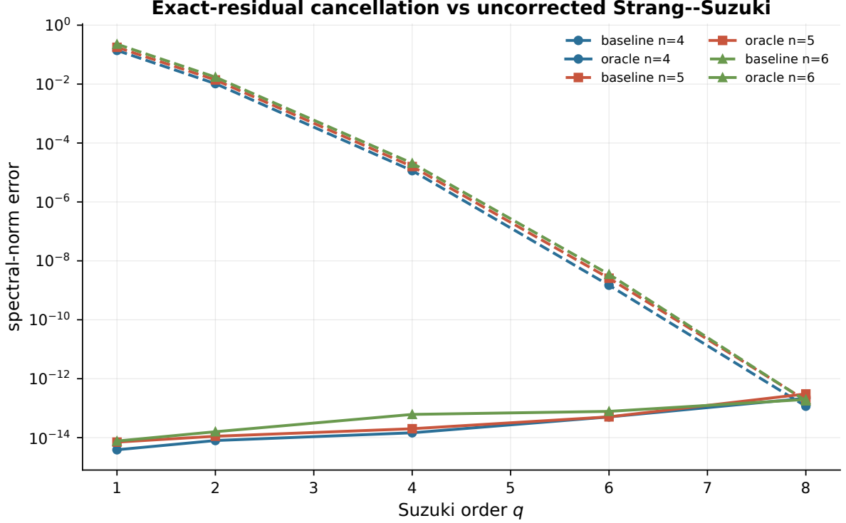
Figure 1. Fixed-time spectral-norm errors for n = 4, 5, 6 and q = 1, 2, 4, 6, 8 . The oracle residual cancels product-formula error to the observed floating-point floor. The highest-order baseline is itself near round-off at this step size.
