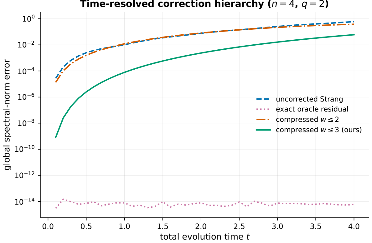
Extended Data Fig. 2 | Time-resolved correction hierarchy for n = 4 , q = 2 , J = h = 1 , and r = 10 . The w \leq 3 projected residual uniformly improves the baseline in this sweep; w \leq 2 is less reliable.
