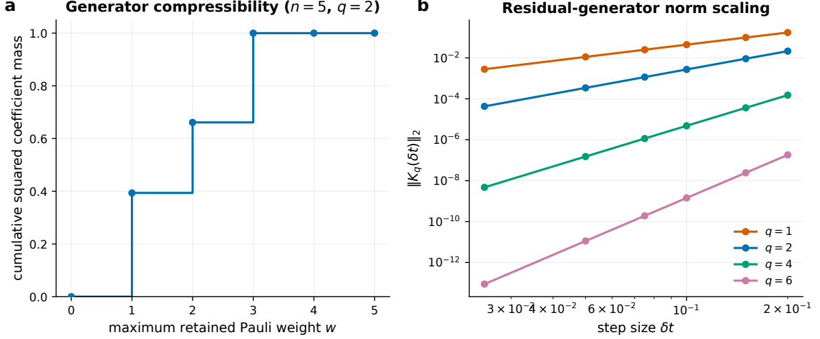
Extended Data Fig. 3 | Structure of the residual generator. a , Cumulative squared Pauli coefficient mass for the n = 5, q = 2 residual generator; weight three captures the dominant leading structure, while higher weights capture subleading BCH terms. b , Residual-generator norm \|K_q(\delta t)\|_2 versus step size for n = 4 and q = 1, 2, 4, 6 ; the norm decreases rapidly with order, consistent with product-formula order conditions and Theorem 3.
