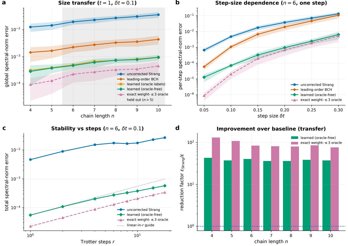
Figure 2. Learned residual generators on the disordered TFIM. Shaded bands are one standard deviation over disordered realizations. a , Global spectral-norm error at t = 1, \delta t = 0.1 versus chain length for the uncorrected Strang step, leading-order BCH, the learned correction trained on oracle labels and on oracle-free patch labels (overlapping), and the exact weight- \leq 3 oracle; the shaded region marks lengths absent from training ( n > 5 ), extending to n = 10 . b , Per-step error versus step size \delta t at n = 6 ; leading-order BCH approaches the uncorrected step as \delta t grows, while the learned correction tracks the oracle. c , Total error versus number of Trotter steps r ( n = 6, \delta t = 0.1 ), growing linearly in r as Theorem 4 predicts (grey guide). d , Oracle-free predicted versus exact coefficients on held-out transfer sizes n = 6, \dots, 10 ( R^2 = 0.9998 ). One per-site network, trained only on n = 4, 5 , sees only local couplings at inference.
