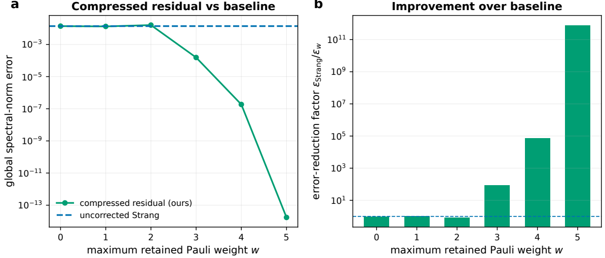
Extended Data Fig. 1 | Compressed-residual compilation for n = 5 , q = 2 . a , Spectral-norm error versus maximum retained Pauli weight w , against the uncorrected baseline. b , Improvement factor over the baseline by weight. The sharp improvement at w = 3 is predicted by the leading-support theorem for the Strang residual (Theorem 8).
