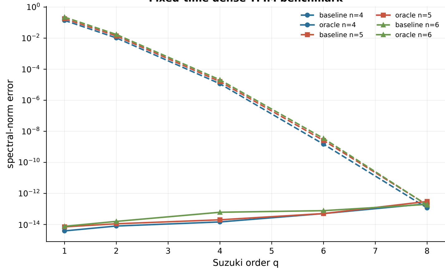
Fixed-time dense TFIM benchmark
