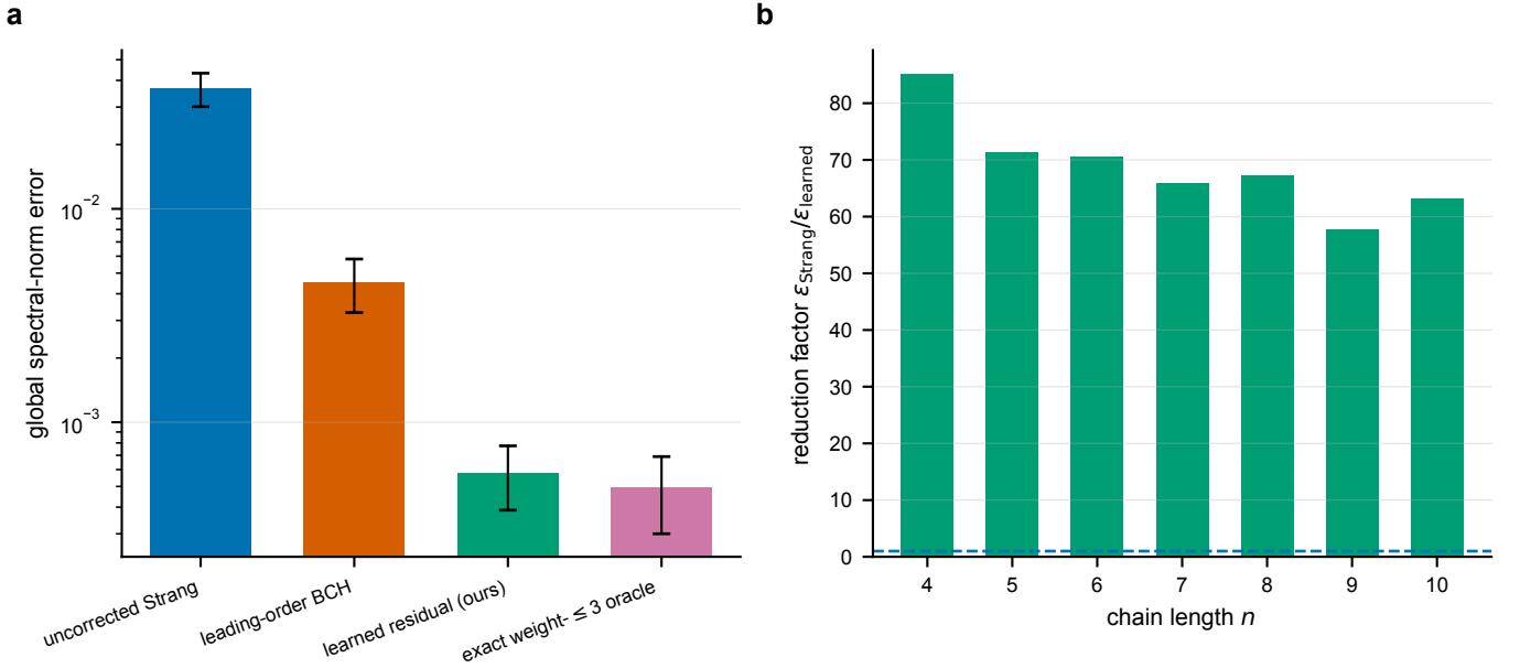
FIG. 6. Proposed learned correction versus all baselines. a , Final global spectral-norm error at the largest held-out transfer size ( n = 10 ) for the uncorrected Strang step, leading-order BCH, the learned residual (ours), and the exact weight- \leq 3 oracle; error bars show one standard deviation over disordered realizations. b , Error-reduction factor \epsilon_{\text{Strang}}/\epsilon_{\text{learned}} of the learned correction over the uncorrected Strang baseline across all chain lengths, including the held-out transfer sizes n \geq 6 .
