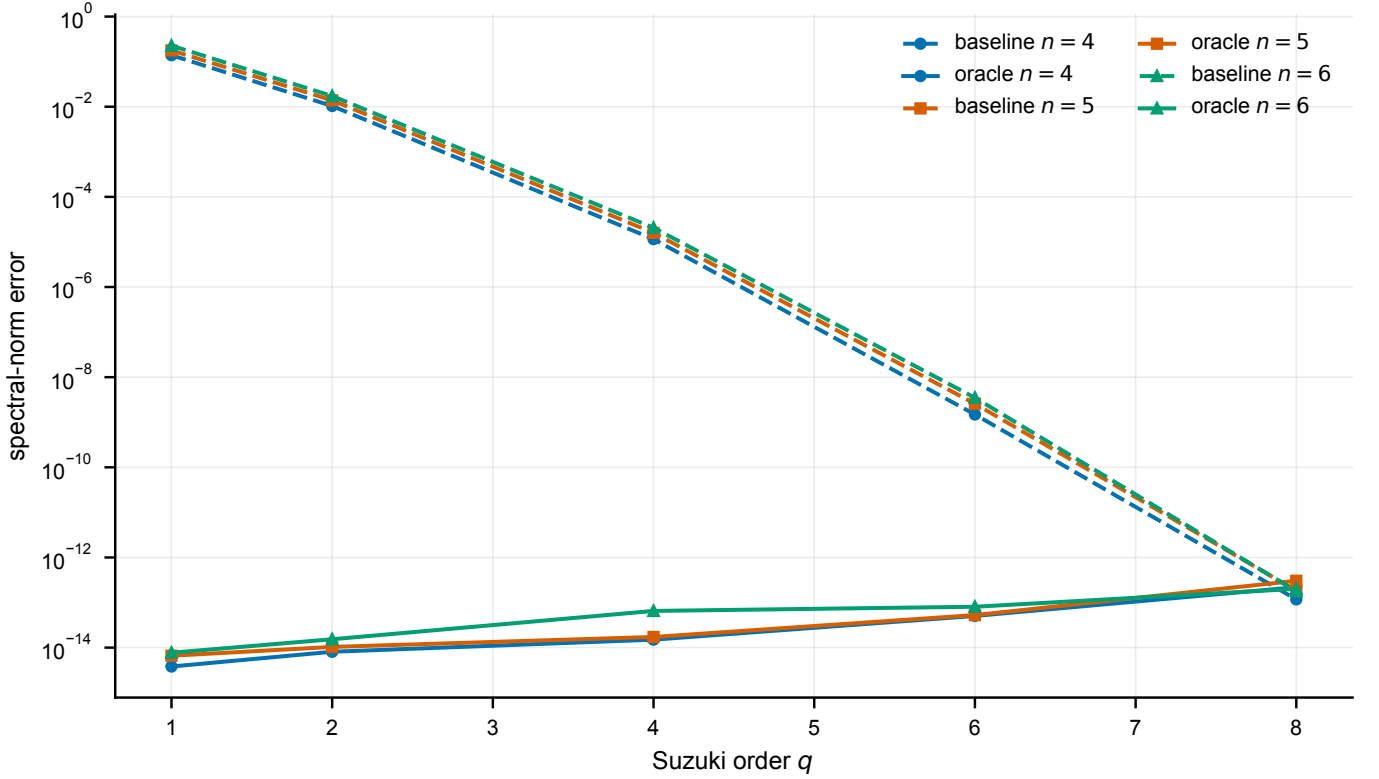
FIG. 2. Fixed-time spectral-norm errors for n = 4, 5, 6 and q = 1, 2, 4, 6, 8 ( J = h = 1 , t = 1 , r = 10 ). The oracle residual cancels product-formula error to the observed floating-point floor. The highest-order baseline is itself near round-off at this step size. Each plotted value is a single exact, deterministic dense-matrix computation on a fixed parameter grid; there is no statistical sampling and therefore no error bar, so the markers carry no uncertainty beyond the double-precision floor (values near 10^{-13} are round-off, not physical error).
