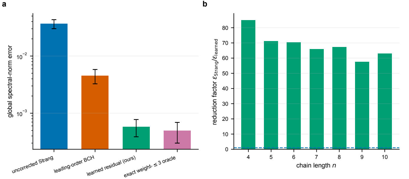
FIG. 6. Proposed learned correction versus all baselines. a , Final global spectral-norm error at the largest held-out transfer size ( n = 10 ) for the uncorrected Strang step, leading-order BCH, the learned residual (ours), and the exact weight- \leq 3 oracle; error bars show one standard deviation over disordered realizations. b , Error-reduction factor \epsilon_{\text{Strang}}/\epsilon_{\text{learned}} of the learned correction over the uncorrected Strang baseline across all chain lengths, including the held-out transfer sizes n \geq 6 .
