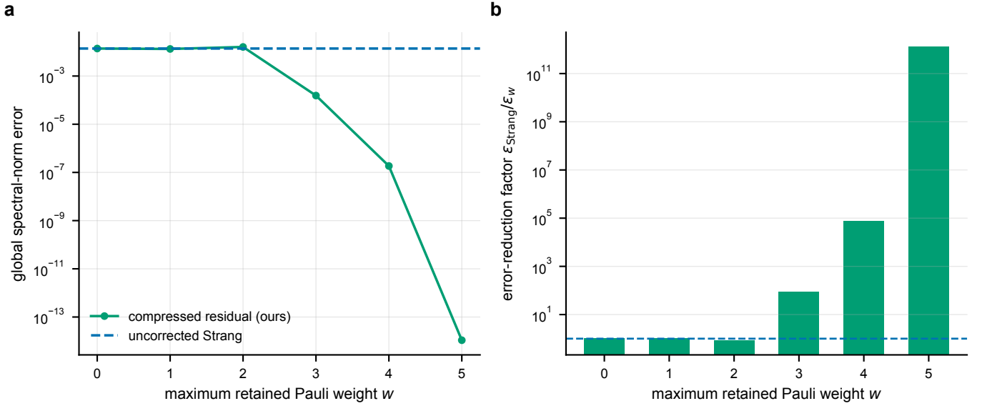
FIG. 7. Compressed-residual compilation for n = 5 , q = 2 ( J = h = 1 , t = 1 , r = 10 ). a , Spectral-norm error versus maximum retained Pauli weight w , against the uncorrected baseline. b , Improvement factor over the baseline by weight. The sharp improvement at w = 3 is predicted by the leading-support theorem for the Strang residual (Theorem 8). All values are exact, deterministic dense-matrix computations (no sampling, hence no error bars); the w = 5 row sits at the double-precision floor.
