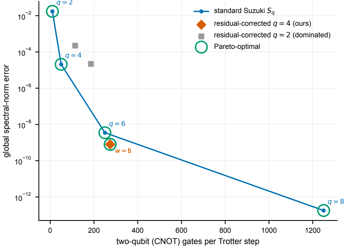
FIG. 4. Residual correction enlarges the product-formula error–cost frontier (open-boundary TFIM, n = 6 , J = h = 1 , t = 1 , r = 10 ). Two-qubit-gate (CNOT) cost per Trotter step versus global spectral-norm error for standard Suzuki steps S_q (blue, labelled by order) and for residual-corrected fourth-order steps with a compiled weight- \leq w correction (orange diamonds). Open green circles mark Pareto-optimal points. The corrected q = 4 , w = 5 step occupies the accuracy gap between standard q = 6 and q = 8 at \approx 1/4.6 of the q = 8 cost. Corrected second-order points (grey squares) are dominated and shown for completeness. All values are exact, deterministic dense-matrix computations.
