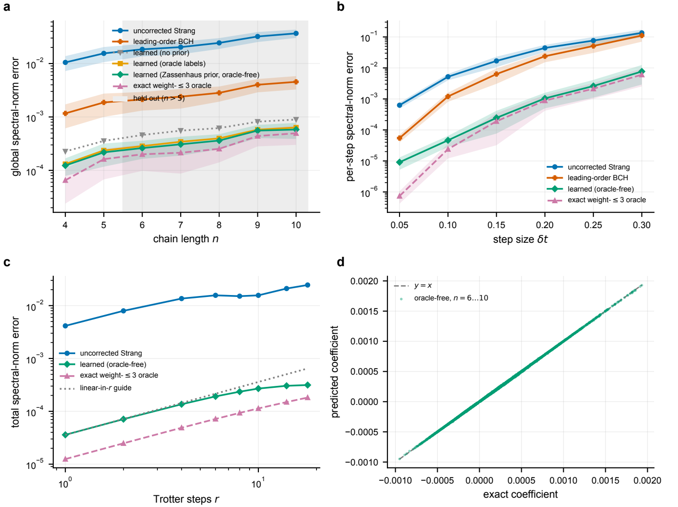
FIG. 5. Learned residual generators on the disordered TFIM. Shaded bands are one standard deviation over disordered realizations. a , Global spectral-norm error at t = 1 , \delta t = 0.1 versus chain length for the uncorrected Strang step, leading-order BCH, the prior-free learned ablation, the learned correction (analytic second-order Zassenhaus prior plus learned residual) trained on oracle labels and on oracle-free patch labels (overlapping), and the exact weight- \leq 3 oracle; the shaded region marks lengths absent from training ( n > 5 ), extending to n = 10 . b , Per-step error versus step size \delta t at n = 6 ; leading-order BCH approaches the uncorrected step as \delta t grows, while the learned correction tracks the oracle. c , Total error versus number of Trotter steps r ( n = 6 , \delta t = 0.1 ), growing linearly in r as Theorem 4 predicts (grey guide). d , Oracle-free predicted versus exact coefficients on held-out transfer sizes n = 6, \dots, 10 ( R^2 = 0.9999 ). One per-site network, trained only on n = 4, 5 , sees only local couplings at inference.
