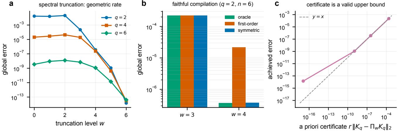
FIG. 3. Spectral truncation of the residual generator: rate, repair, and certificate (open-boundary TFIM, J = h = 1 , t = 1 , r = 10 ). a , Global spectral-norm error of the level- w truncated residual compilation \hat{G}_{q,w} versus truncation level w at n = 6 , for base orders q = 2, 4, 6 ; beyond the effective threshold the error decays geometrically (Theorem 10; per-level factors in Table III). b , The truncated correction’s gate-level error at n = 6 , q = 2 : the first-order inner compilation (Theorem 11) stalls above the dense oracle, while the symmetric inner compilation (Theorem 12) recovers it, repairing the structural floor. c , The a priori certificate r\|K_q - \Pi_w K_q\|_2 versus the achieved error across levels ( n = 6 , q = 2 ); every point lies on or above the diagonal, so the certificate is a valid upper bound and selects the truncation bandwidth from the target accuracy alone. All values are exact, deterministic dense-matrix computations.
