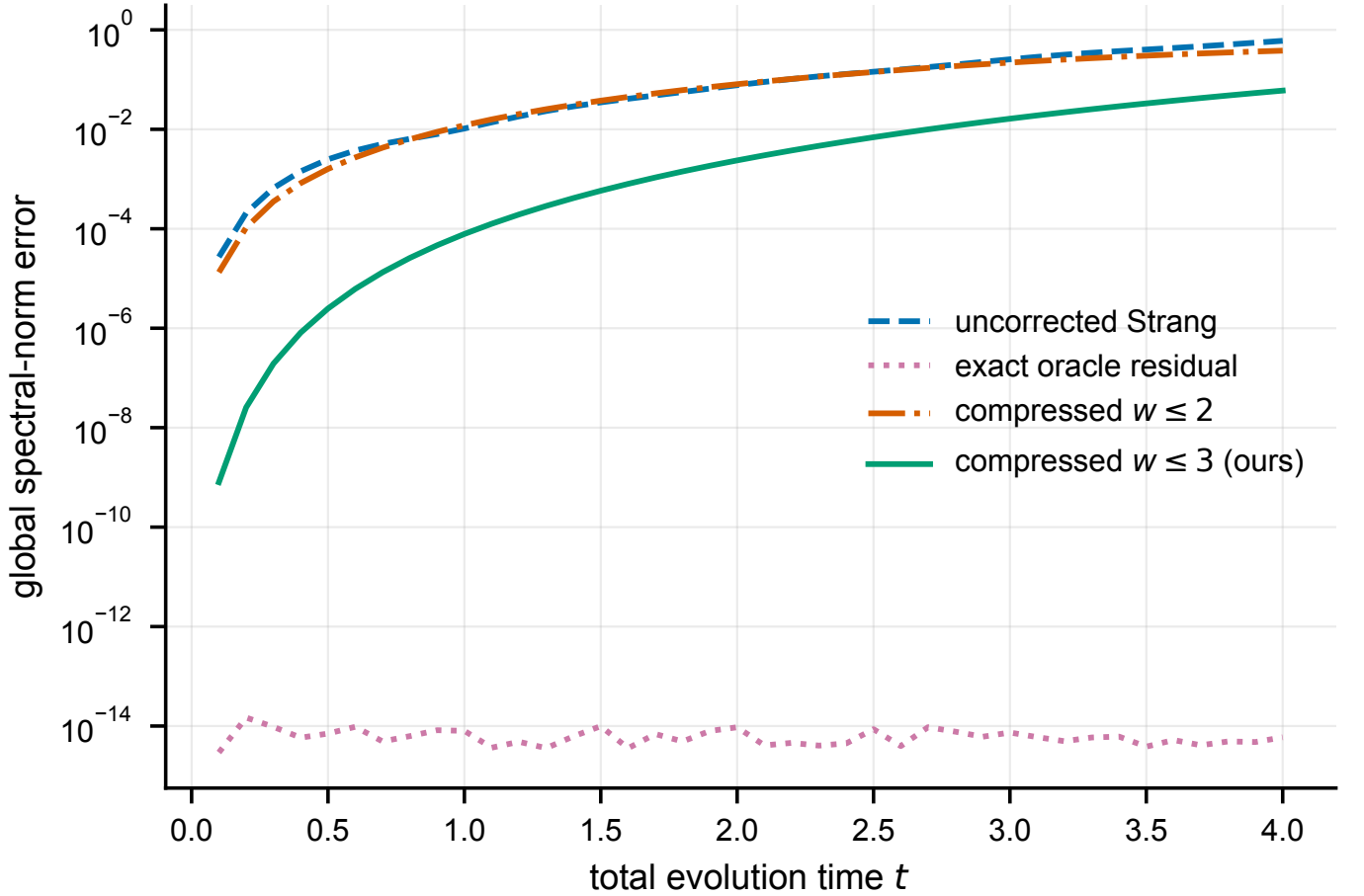
FIG. 8. Time-resolved correction hierarchy for n = 4 , q = 2 , J = h = 1 , and r = 10 , over 40 total times t \in [0.1, 4.0] . The w \leq 3 projected residual uniformly improves the baseline in this sweep; w \leq 2 is less reliable. Each curve is an exact, deterministic dense-matrix computation (no sampling, hence no error bars).
