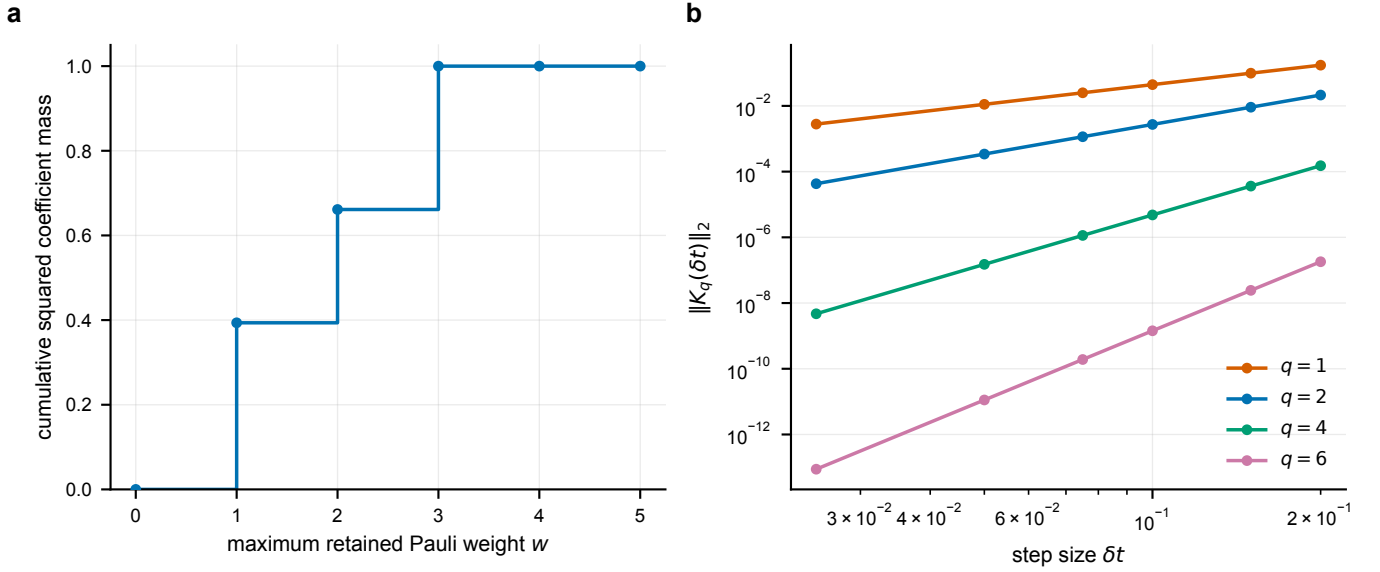
FIG. 9. Structure of the residual generator. a , Cumulative squared Pauli coefficient mass for the n = 5 , q = 2 residual generator at \delta t = 0.1 ; weight three captures the dominant leading structure, while higher weights capture subleading BCH terms. b , Residual-generator norm \|K_q(\delta t)\|_2 versus step size for n = 4 and q = 1, 2, 4, 6 ; the norm decreases rapidly with order, consistent with product-formula order conditions and Theorem 3. Both panels are exact, deterministic dense-matrix computations (no sampling, hence no error bars).
