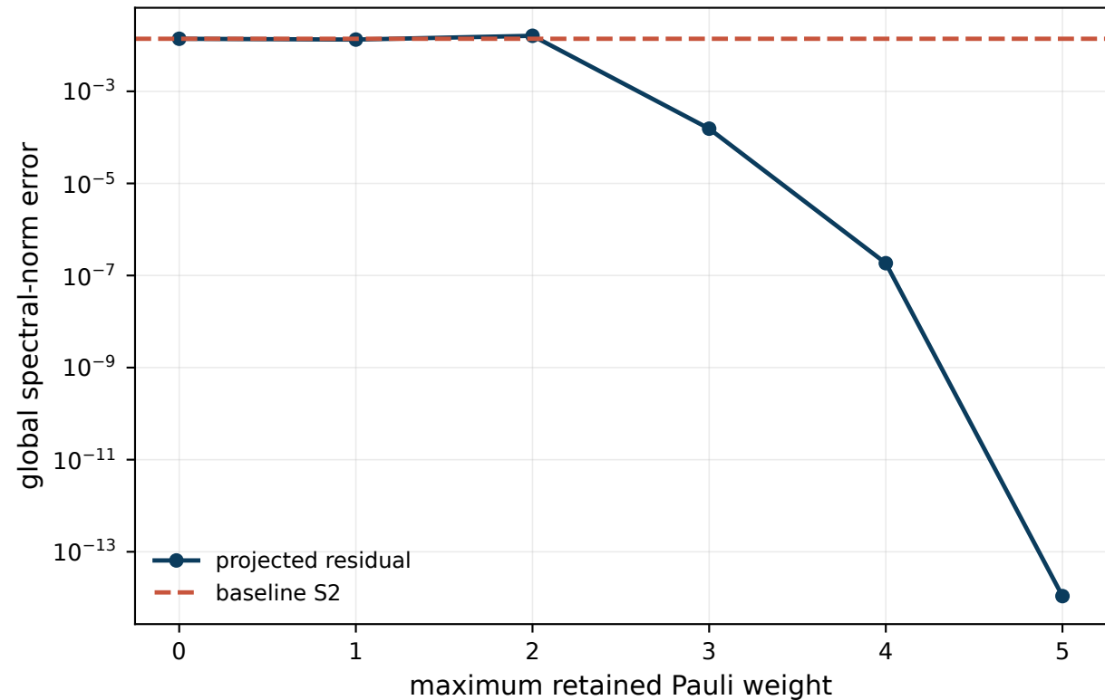
Projected residual compilation, n=5 , q=2
