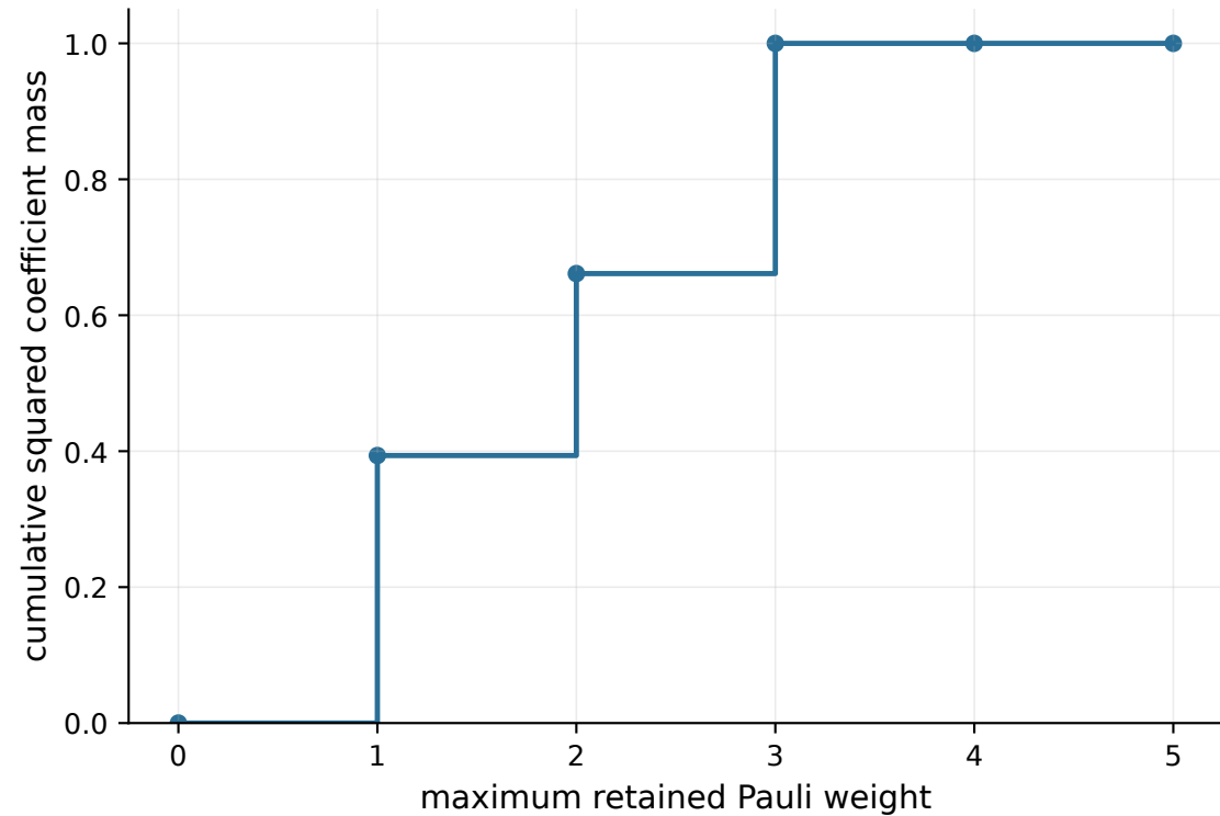
Residual-generator compressibility, n=5 , q=2
