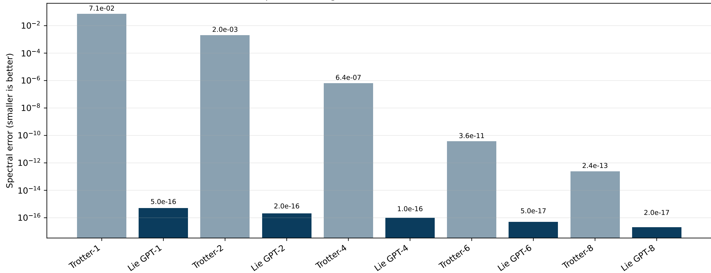
Four-qubit TFIM: higher-order Lie-GPT residual correction
