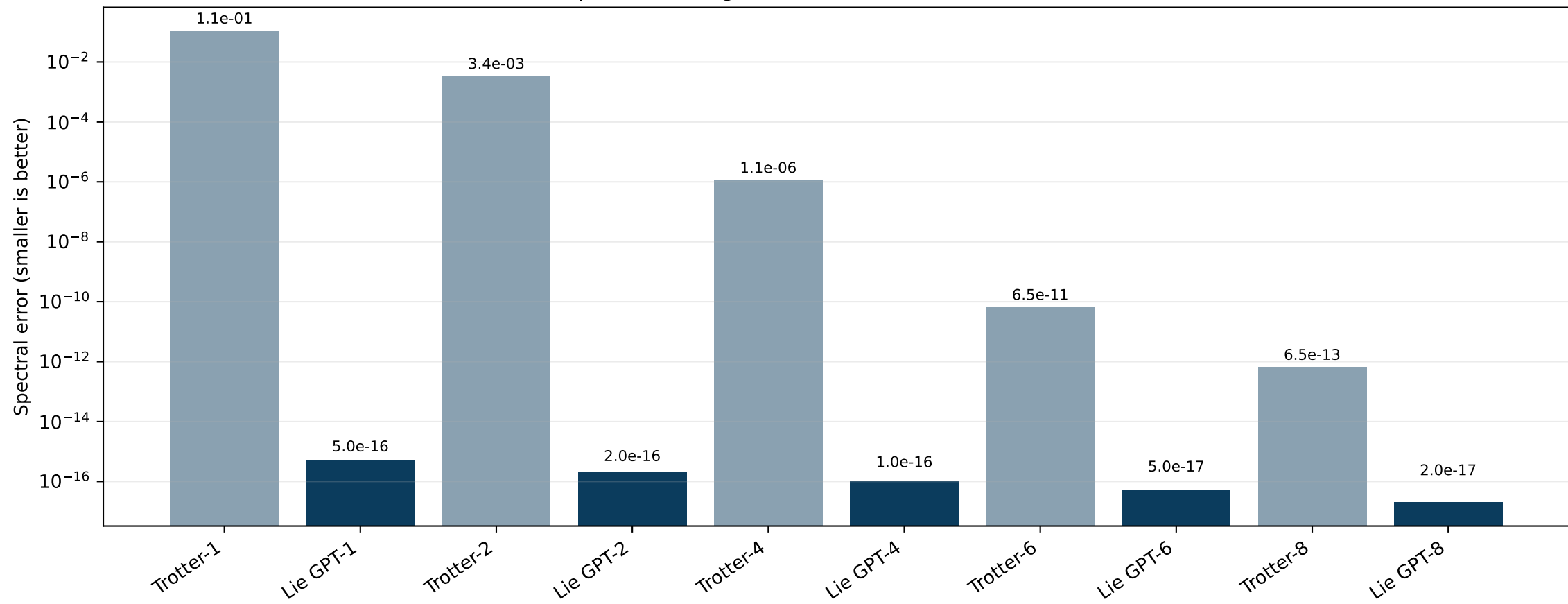
Six-qubit TFIM: higher-order Lie-GPT residual correction
