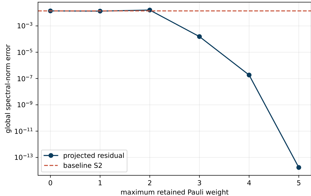
Projected residual compilation, n=5 , q=2
