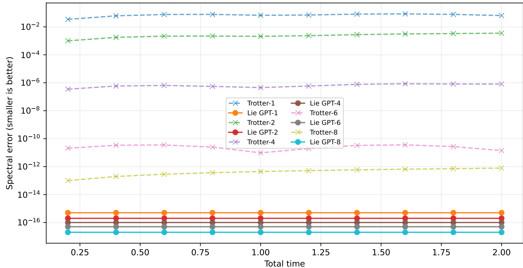
Four-qubit time sweep: Lie-GPT below same-order Trotter
