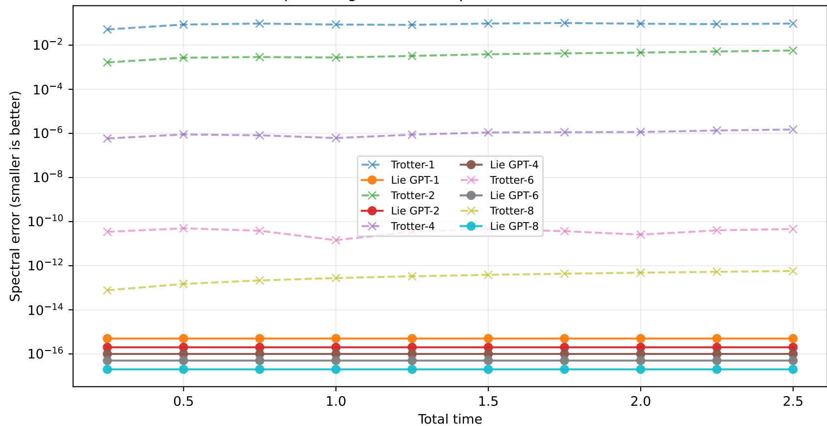
Five-qubit longer-time sweep: dense residual Lie-GPT
