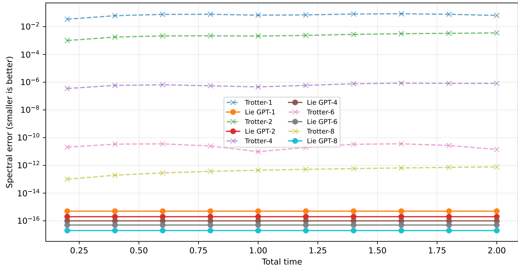
Higher-order diagnostic: Lie-GPT residual correction
