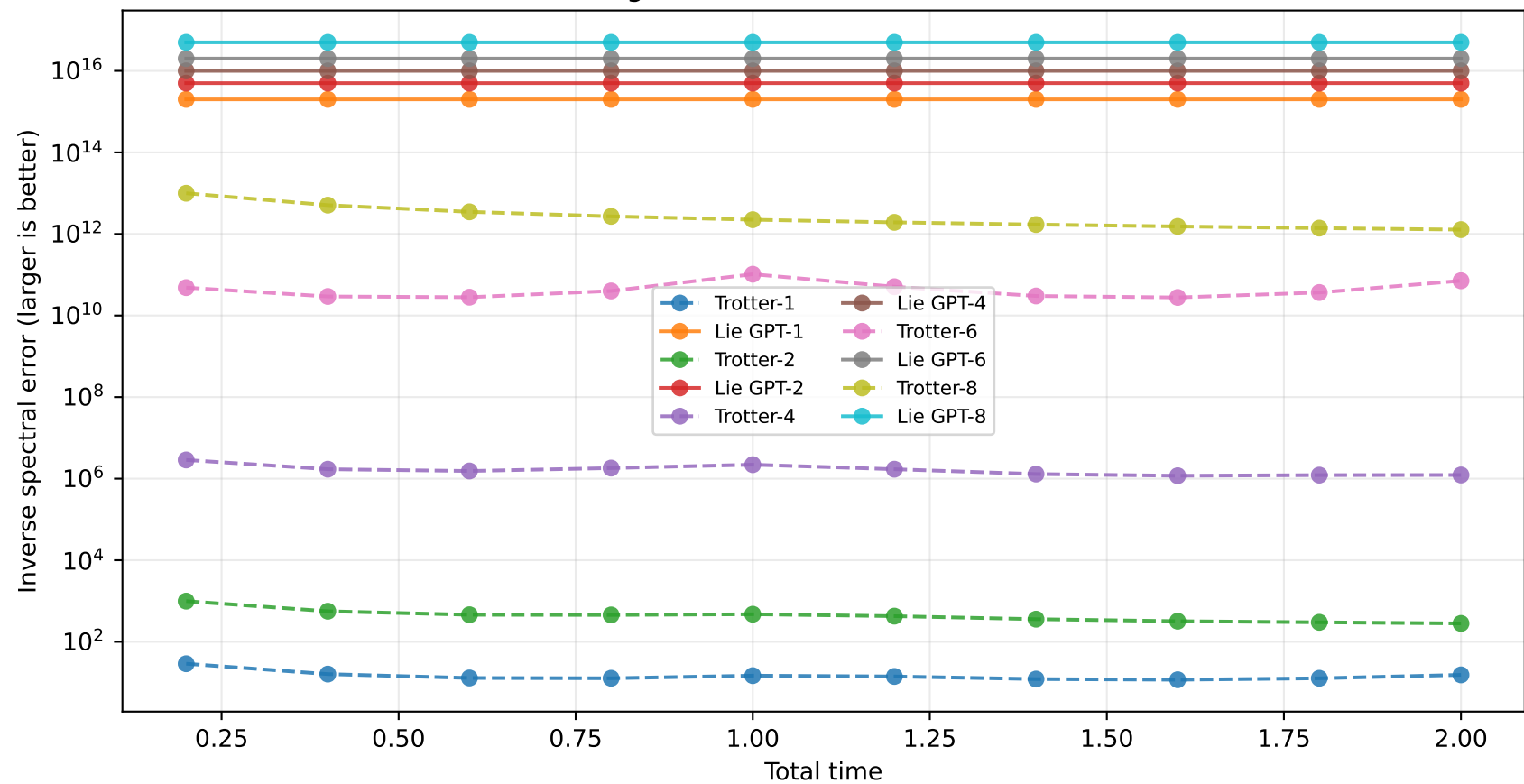
Inverse-error score: higher-order Lie-GPT dominates same-order Trotter
