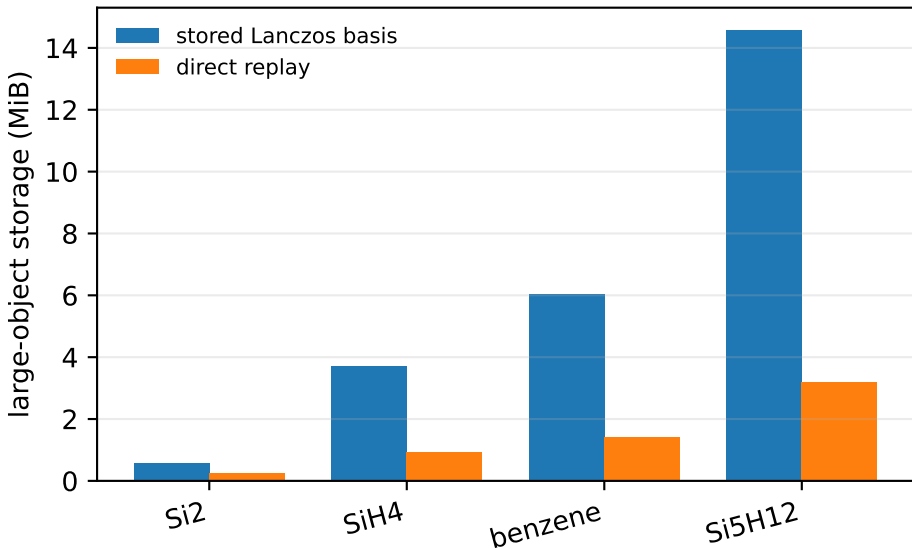
Measured allocation ledger at m = 48
