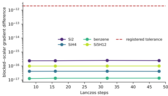
Figure 1: Finite-objective equivalence across four authenticated matrices and four depths. The ordinate is the Euclidean difference between full-block and parameterwise gradients. Every value is at roundoff scale and below the registered 2 \times 10^{-12} tolerance.
