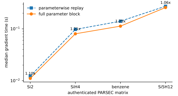
Figure 2: Median gradient time from nine alternating repetitions. Labels give the scalar-to-block ratio. Accuracy is checked separately in Figure 1.
