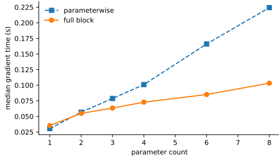
Figure 4: Measured SiH4 parameter scaling. Full blocking gives a small timing difference at one and two parameters and an increasing separation thereafter. The curve is a host-specific consequence of the exact launch ledger.
