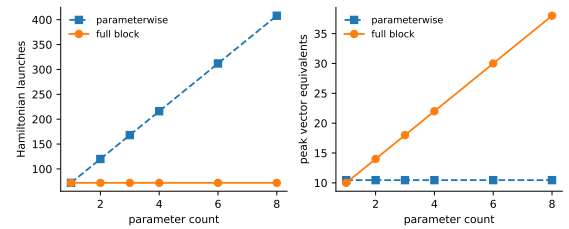
Figure 3: Exact ledger on SiH4 at m = 24 . Full blocking holds Hamiltonian launches at 3m = 72 as p grows, compared with (1 + 2p)m for parameterwise replay. The reduction is purchased with an ambient-vector ledger that grows linearly in p .
