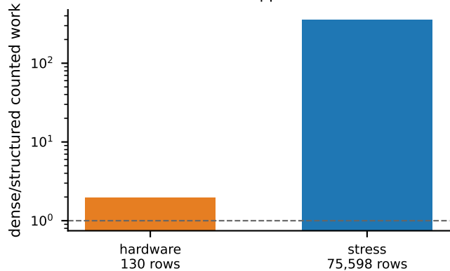
batched application
