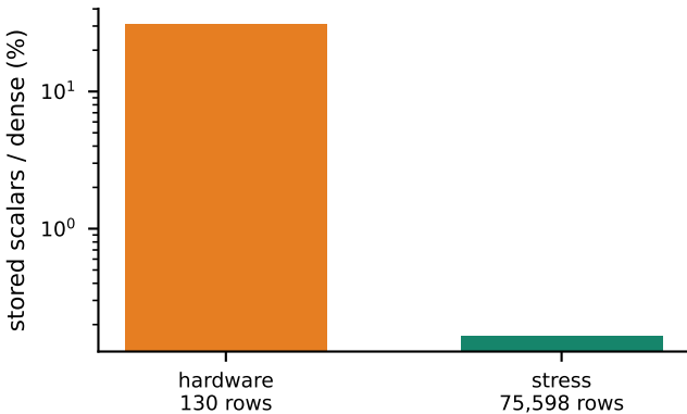
matrix-free storage
