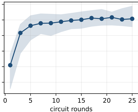
confirmation decoder
