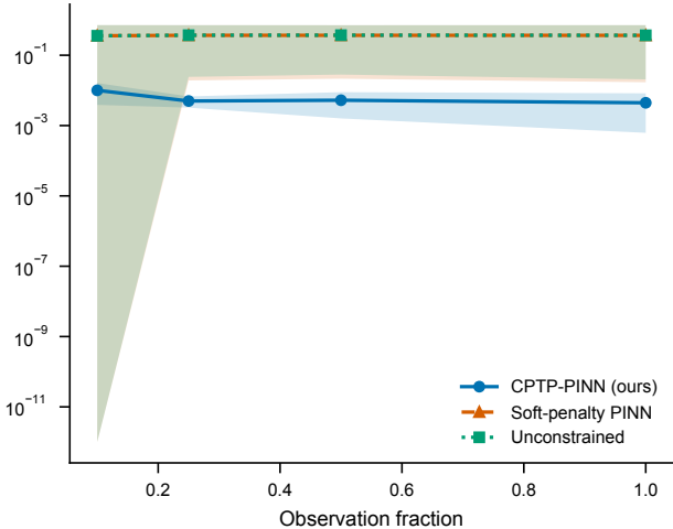
Mean trace distance
