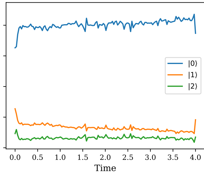
CPTP-PINN Prediction
