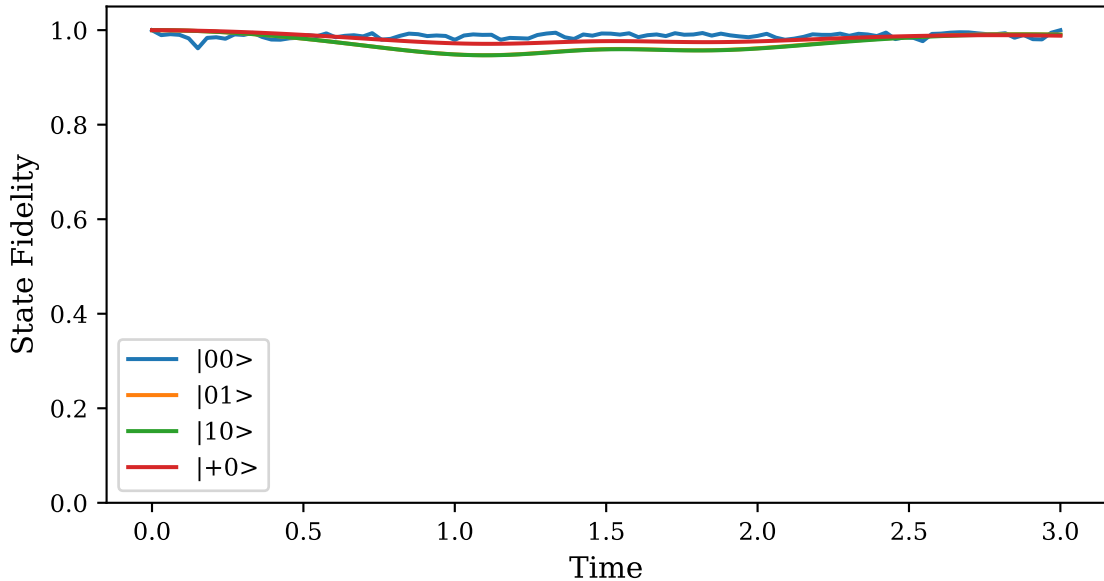
Two-Qubit Gate: State Fidelity Proxy
