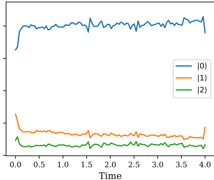
CPTP-PINN Prediction
