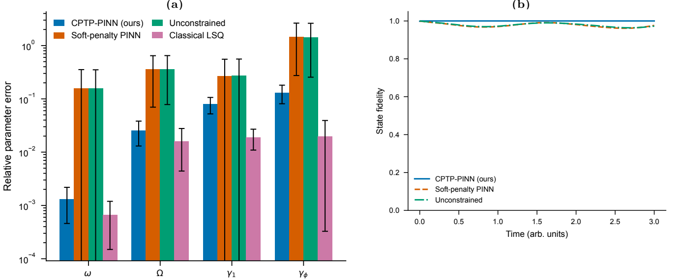
FIG. 2. Single-qubit system identification. (a) Relative parameter-recovery error per method (mean and 95% confidence interval over five seeds, log scale): the CPTP-PINN strongly outperforms the soft-penalty and unconstrained networks and is competitive with a classical least-squares fit that already knows the exact model (Table I). (b) State fidelity between the learned and exact density-matrix trajectories (representative seed); the hard-constrained CPTP-PINN stays inside \mathcal{D}(\mathcal{H}) by construction. Error bars and bands are 95% confidence intervals over five random seeds.
