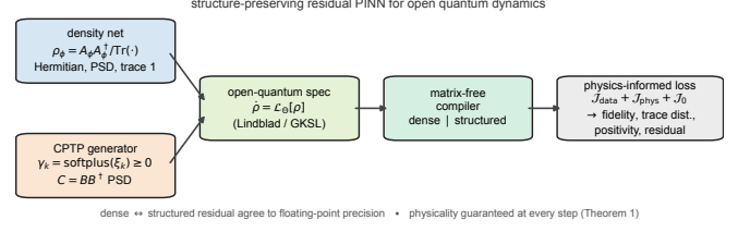
FIG. 1. The structure-preserving, physics-informed framework. Two structure-preserving networks feed a physics-informed residual. The density network maps time to a lower-triangular factor A_\phi(t) and outputs \rho_\phi = A_\phi A_\phi^\dagger / \text{Tr}(A_\phi A_\phi^\dagger) , which is Hermitian, positive semidefinite, and unit trace at every time and every training step (Theorem 1); the generator is parameterized so that all Lindblad rates are nonnegative [\gamma_k = \text{softplus}(\xi_k) \geq 0] or the Kossakowski matrix is positive semidefinite [C = BB^\dagger] , keeping \mathcal{L}_\Theta in GKSL form (Theorem 3). A matrix-free compiler lowers the specification \dot{\rho} = \mathcal{L}_\Theta[\rho] to a dense d^2 \times d^2 Liouvillian or a structured residual kernel (the two agree to floating-point precision; Theorem 6). Training minimizes a physics-informed loss combining the masked data term, the Lindblad residual, and the initial condition; the outputs are a physically valid trajectory, a completely positive generator, and the metrics (state fidelity, trace distance, positivity-violation rate, and the trace-norm residual certificate of Theorem 4). The figure is generated programmatically by ctpcpinn/plotting.py:plot_schematic .
