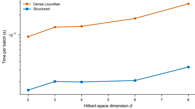
FIG. 4. Matrix-free compiler scaling. Dense superoperator residual-evaluation time versus structured matrix-free evaluation (median over 50 repeats, log scale). The structured path avoids materializing the d^2 \times d^2 Liouvillian; its robust advantage is memory [ O(md^2) versus O(d^4) ], not speed—the dense timings shown rebuild the Liouvillian per state and so overstate any wall-clock gap (see text and Table V).
