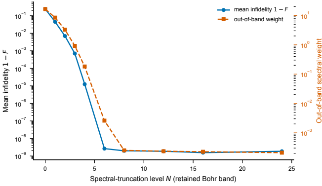
FIG. 5. Operator-system spectral truncation of the open-system generator. Mean infidelity 1 - F of the propagated level- N truncated interaction-picture generator (left axis) and the out-of-band spectral weight \eta_N = \sum_{|k|>N} \|\mathcal{L}_k\| of Theorem 8 (right axis, log scale) versus the retained Bohr-band level N , for a driven dissipative two-qubit system. N=0 is the secular (Davies) generator, N=1 the rotating-wave approximation, and the full band recovers the exact generator (and the structured kernel) to floating-point precision. The certificate \eta_N tracks and bounds the infidelity, decreasing monotonically to zero. Deterministic (no seed averaging).
